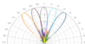
Figure 2: Radiation patterns for various multibeam antennas
