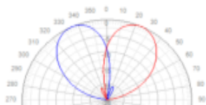
Two Beam antenna for three sector to six sector conversion
