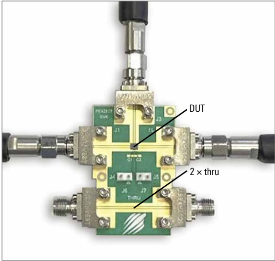
Fig. 2: Example test coupon with a 2× thru configuration. The input and output lines of the DUT to be deembedded are duplicated as reference paths on the same PCB as the DUT so they have the same transmission characteristics as the actual input and output lines, which is a prerequisite for accurate deembedding.
