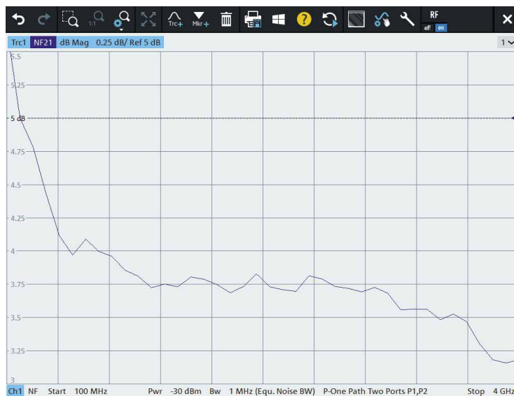
Fig. 2: Noise figure measurement result with the R&S®ZNA26 or R&S®ZNA43.
