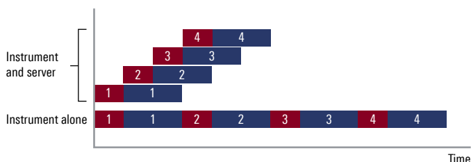
Fig. 1: The two measurement steps – data capture (red) and data analysis (blue) – usually run sequentially in the signal analyzer. New data capture is paused during the analysis phase, as otherwise the buffer would quickly overflow. If the measurement data is sent in real time to a server with sufficient processing power for evaluation, the instrument can constantly capture data and utilize its full acquisition speed. The 2:1 ratio between processing and capture times assumed in this example can be significantly larger in practice, which makes splitting the tasks even more worthwhile.
