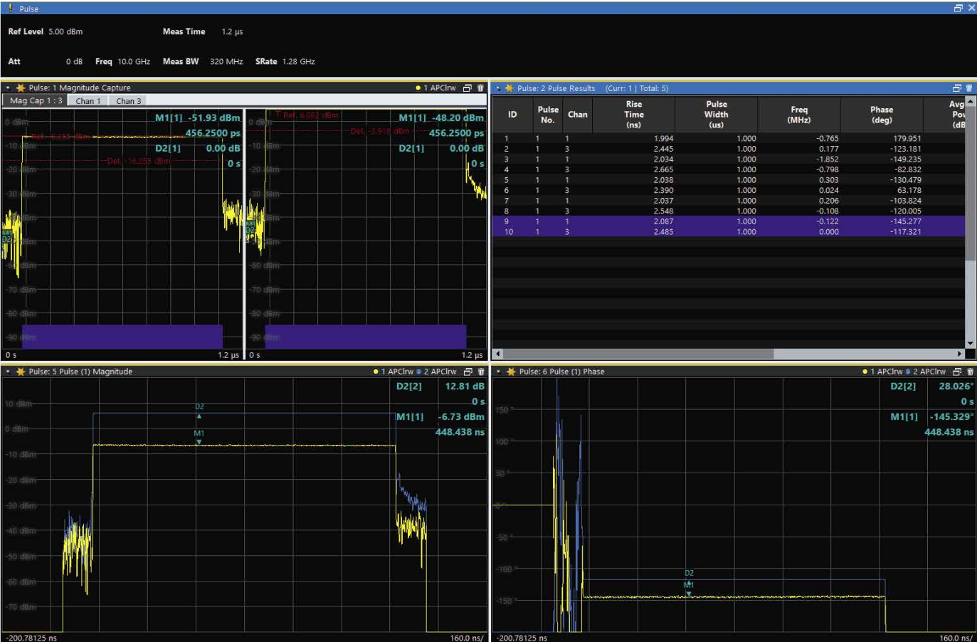
Fig. 6: Using the R&S®VSE software to analyze the example airborne radar signal on the simulated outputs of a dual-channel radar warning receiver. R&S®VSE automatically measures the radar parameters and displays them in tabular form. Phase and amplitude differences can be determined in detail using markers (lower screenshots).
