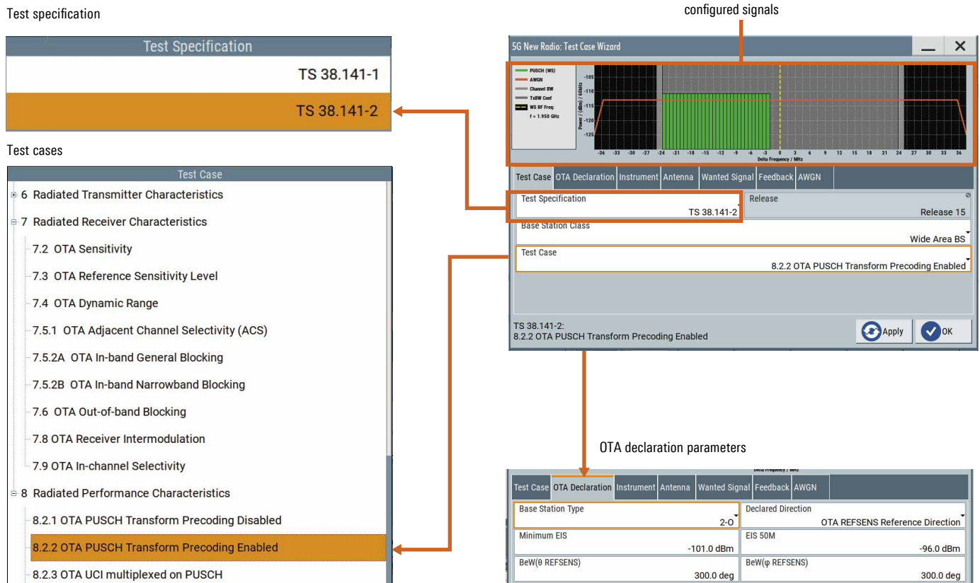
Fig. 3: Test case wizard details. Complex test signals can be composed in just a few steps.
