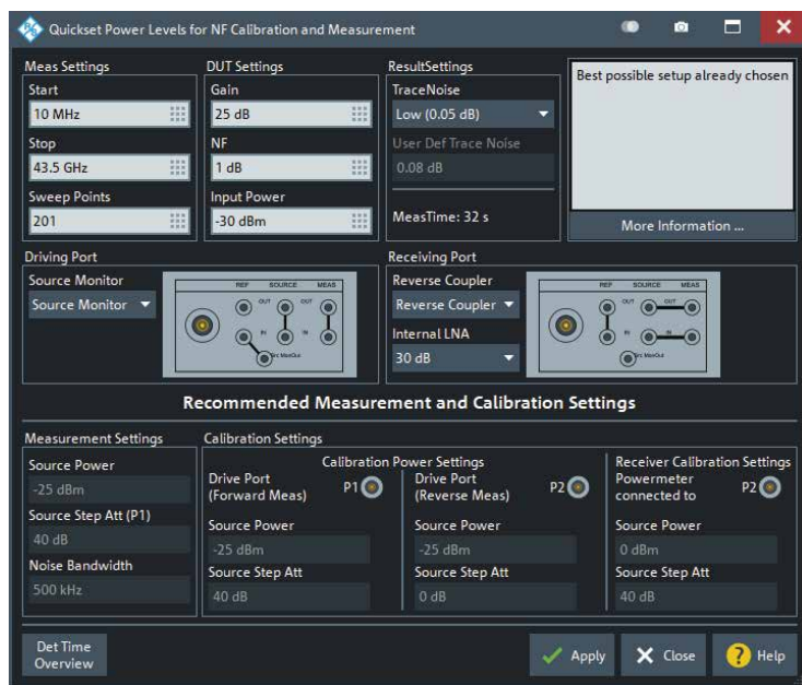
Fig. 1: Noise figure measurement configuration menu. If options such as preamplifier and source monitor are installed (as in this case), they are included in the configuration menu.
