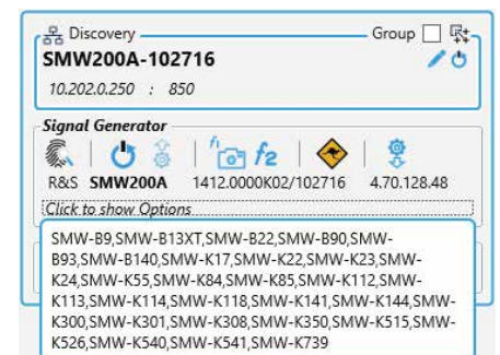
Fig. 4: The fingerprint function in a MINX tile generates a list of all installed options of the instrument concerned. The "Skipky" (SCPI) kangaroo and user definable function keys can be used to save and run remote control command sets, allowing instruments to be configured according to the user's needs at the touch of a button.
