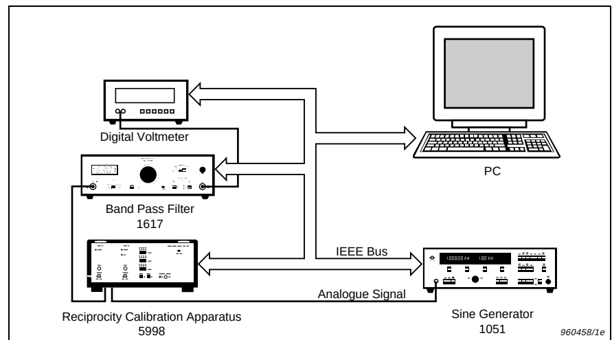
Fig.1 Instrument interconnection in a Reciprocity Calibration System Type 9699
