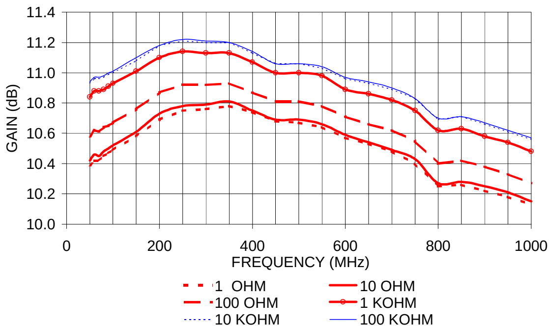
Figure 32 – HELA-10B Gain at Several Values of Shunt Resistance 50-ohm System
