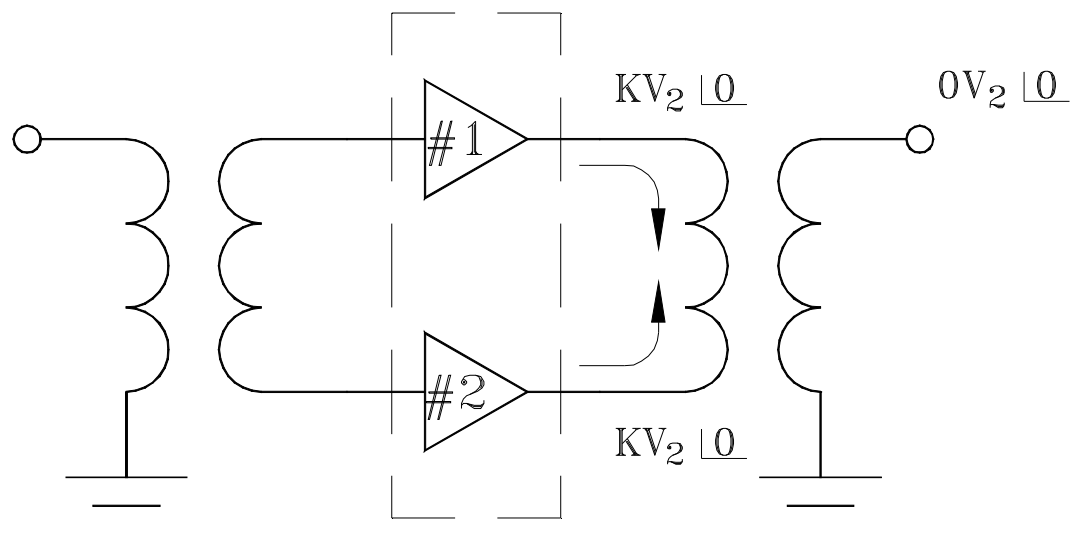
Figure 4 – Second Harmonics Cancel
