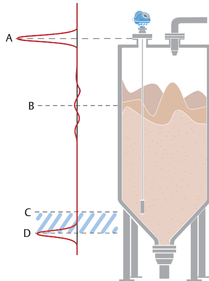
Figure 8. Probe End Projection
