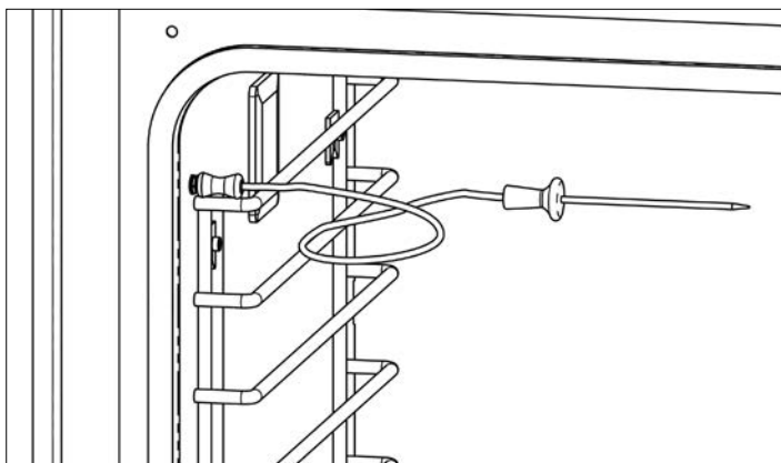
36" OVEN SHOWN
