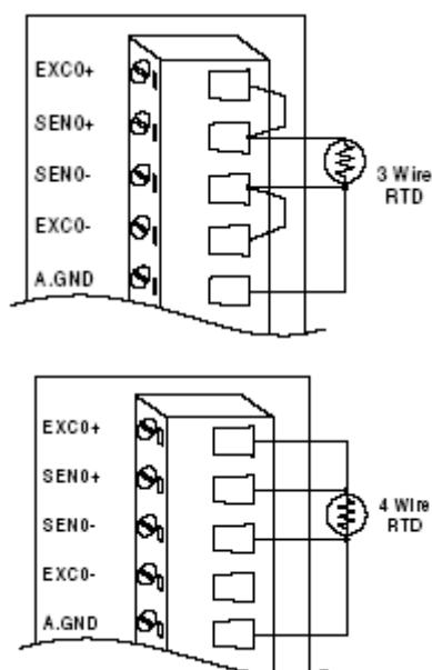
Figure 1.2 RTD Inputs
