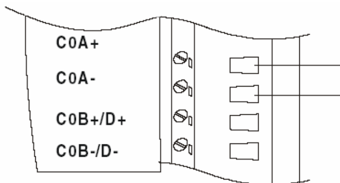
Figure 6.17 Wiring for Frequency Mode
