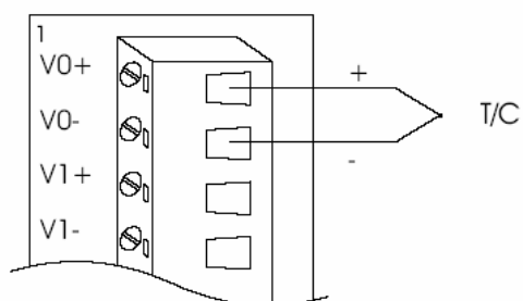
Figure 1.24 Thermocouple Input
