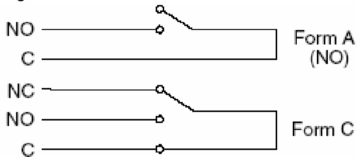
Figure 5.2 Relay Output
