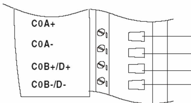
Figure 6.5 Wiring for Up/Down Counting
