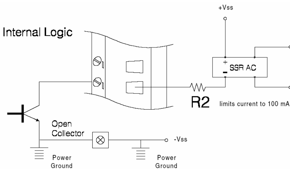
Figure 4.5 Digital Output with SSR (ADAM-5050/5056)
