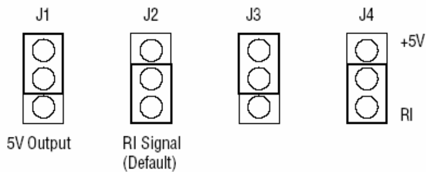
Figure 7.4 Jumper Settings
