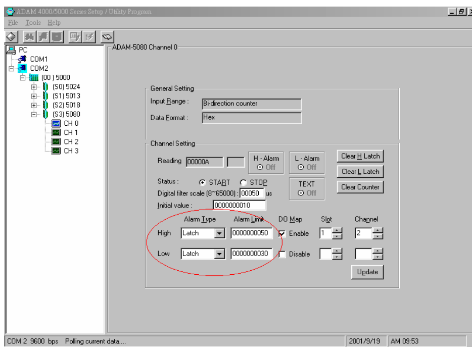
Figure 6.8 Setting Alarm Limit
