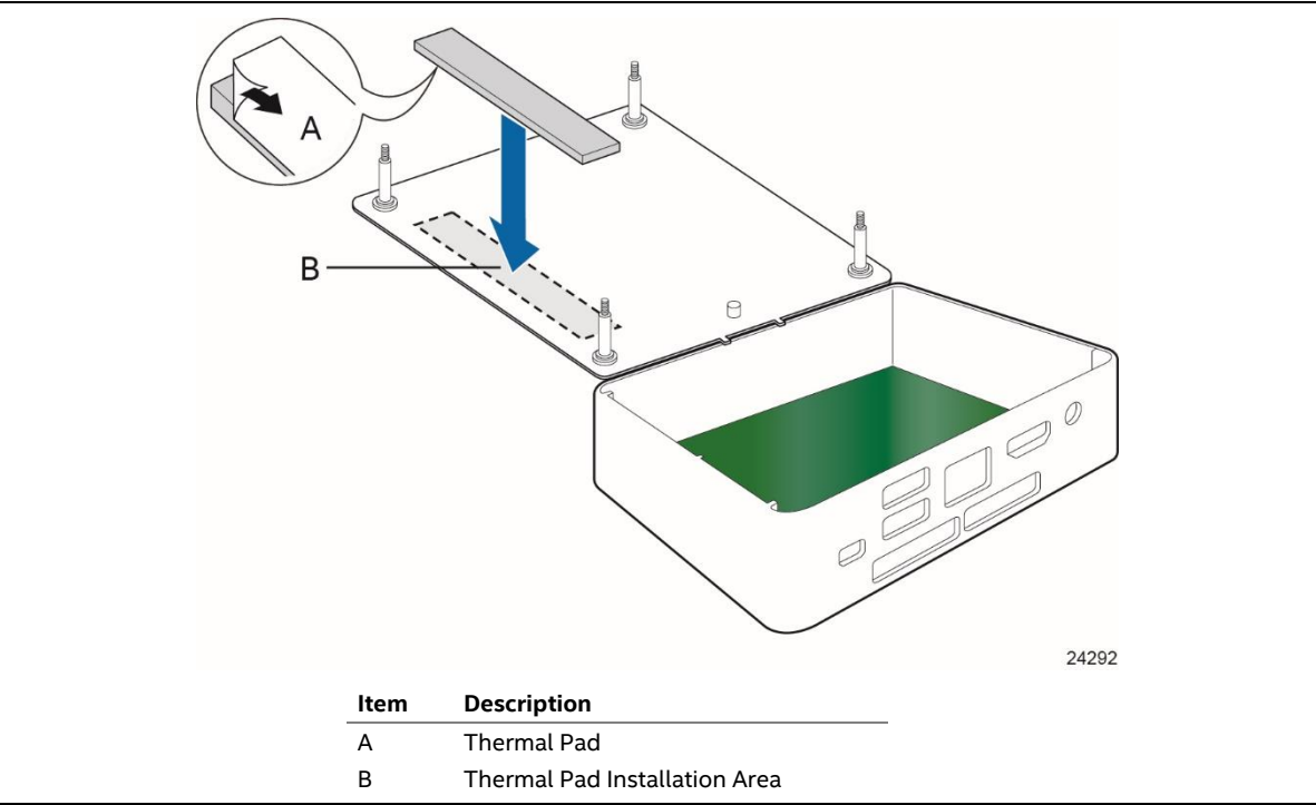
Figure 20. Installation Area of Thermal Pad for Intel NUC Kit NUC7i5BNK
