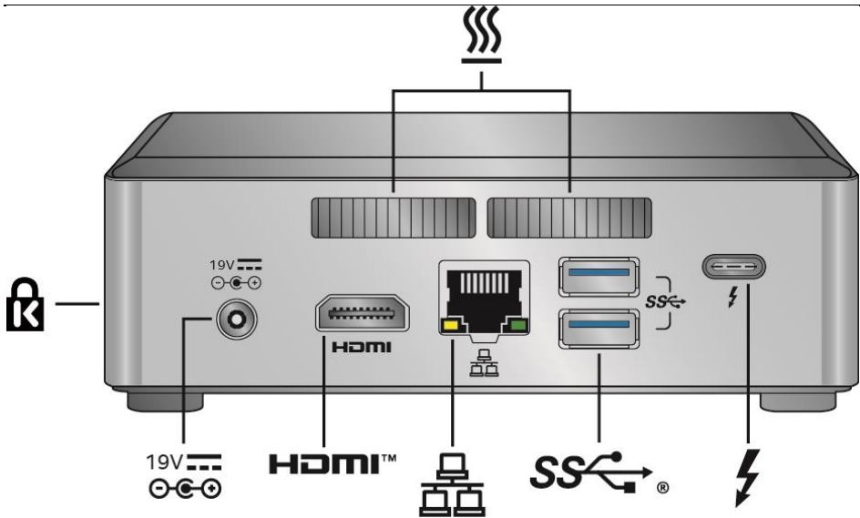
Figure 25. Intel NUC Kit NUC7i5BNK Features – Rear
