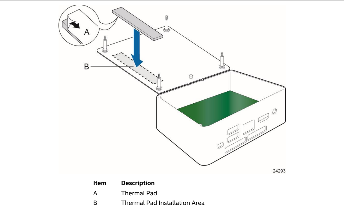
Figure 21. Installation area of Thermal Pad for Intel NUC Kit NUC7i5BNH/NUC7i7BNH
