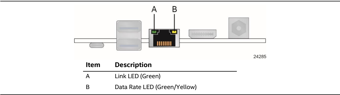
Figure 6. LAN Connector LED Locations
