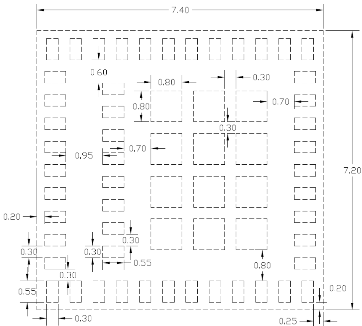
<Top View>
