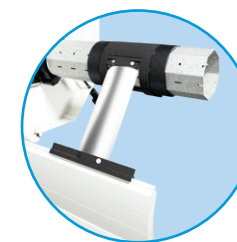
Standard Locking System Plastic and steel locking straps secure your standard SeceuroGlide LT.
