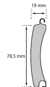
Side Slat Profile
