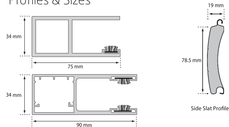
SeceuroGlide Original: Anthracite Colour Finish
