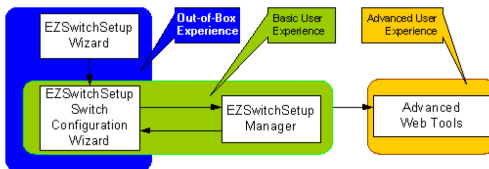
FIGURE 1 EZSwitchSetup components
