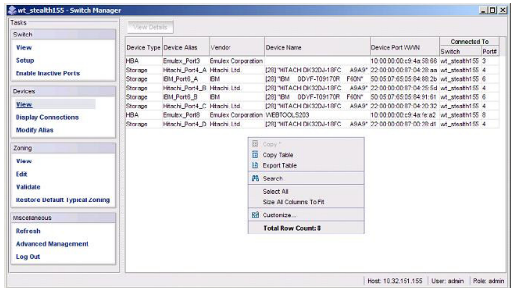
FIGURE 34 Devices view
