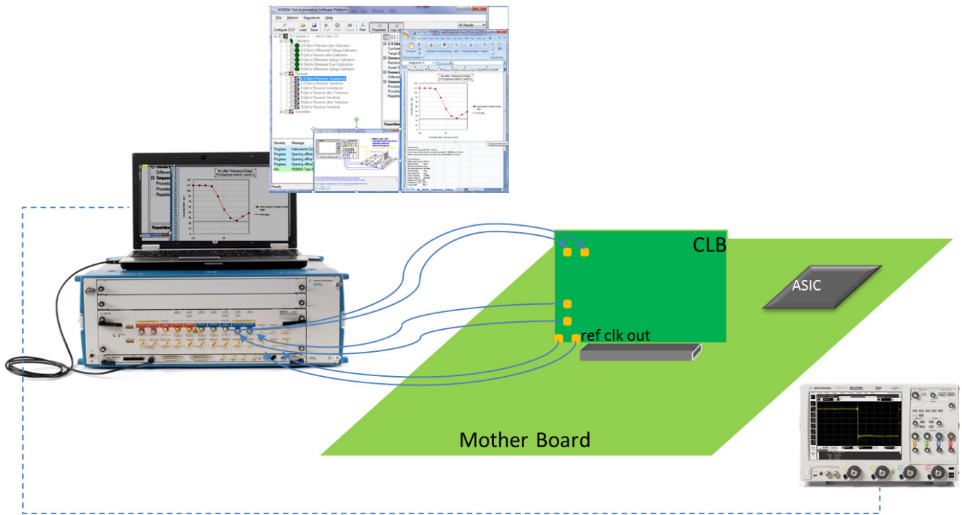
Figure 2: M8020A streamlines complex receiver test setups. The example shows a PCIe 3 (8 GT/s) mother board RX test with J-BERT M8020A connected via a compliance load board (CLB). J-BERT M8020A provides built-in de-emphasis, jitter sources, common-mode and differential mode interference (CMI, DMI), reference clock multiplier, clock recovery and continuous time linear equalizer (CTLE) – everything that is needed is built-in and calibrated.
