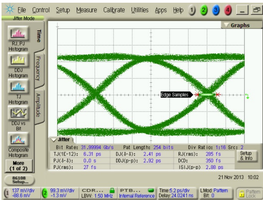
Figure 7. The 32.0 Gb/s output signal shows excellent intrinsic random jitter. This shows the output of the M8061A multiplexer when used with M8041A and its internal clock source (preliminary).
