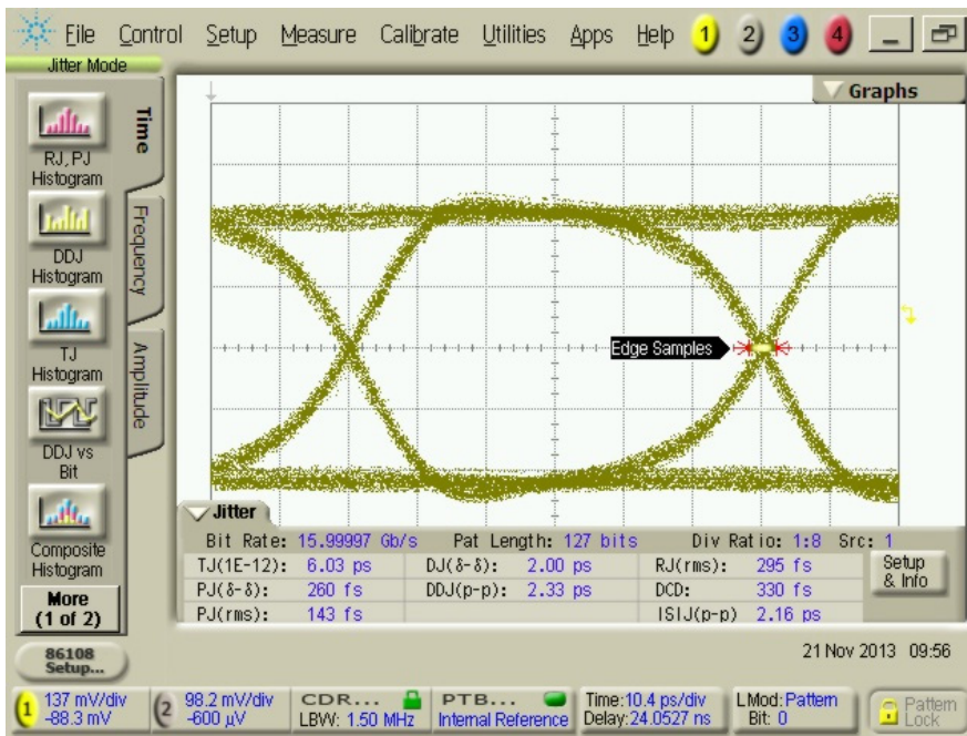
Figure 6. Clean 16.0 Gb/s output signal of J-BERT M8020A with a M8041A 16 Gb/s BERT module using its internal clock source (preliminary).
