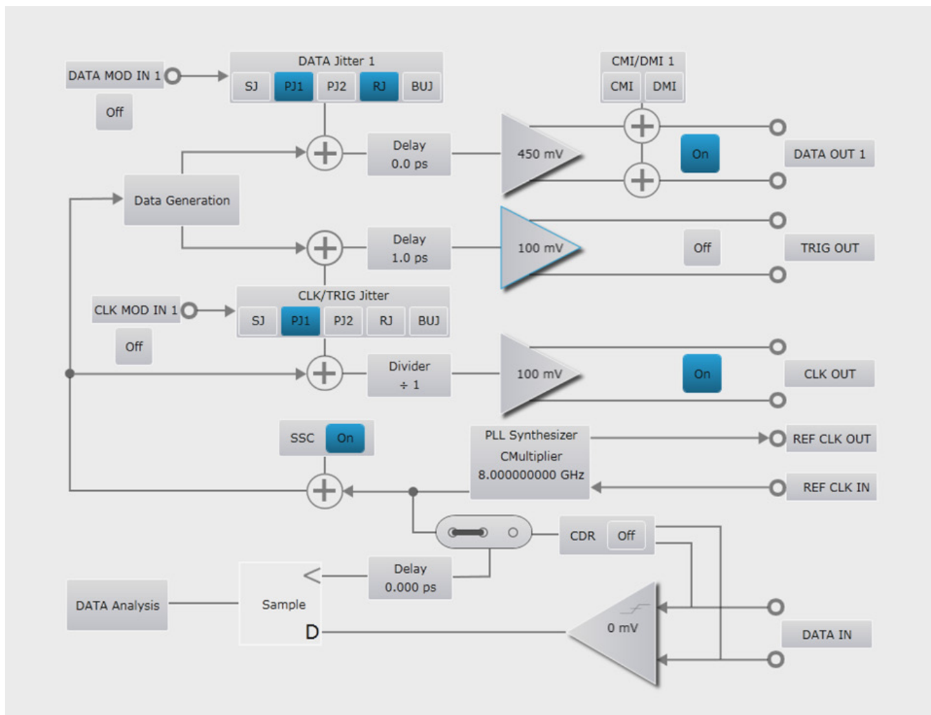
Figure 11. J-BERT M8020A system view for 1 channel, preliminary version.
