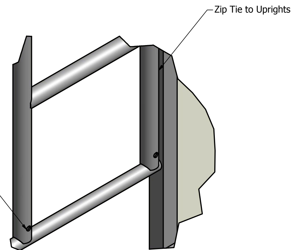
DETAIL D SCALE 1/5
