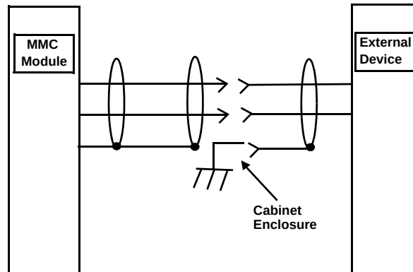
Figure 5-3: Connecting Shielded Cable
