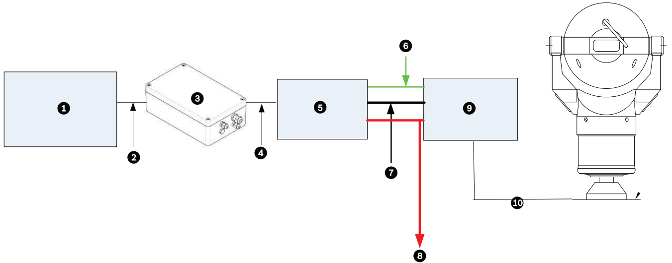
Figure 4.3: MIC PSU Extension with two (2) user-supplied junction boxes (weatherproof or explosion-proof, depending on model and physical location)
