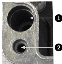
Figure 9.3: Holes for screws for mounting enclosure mounting; holes for screws for enclosure lid
