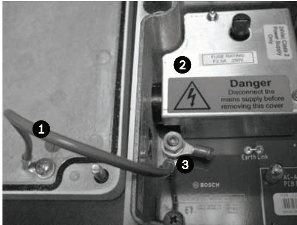
Figure 9.4: Enclosure showing shield and earth core cable between earth terminal post and enclosure lid
