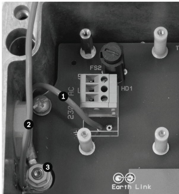
Figure 9.5: Mains input with shield removed, showing terminal block HD1 before wiring
