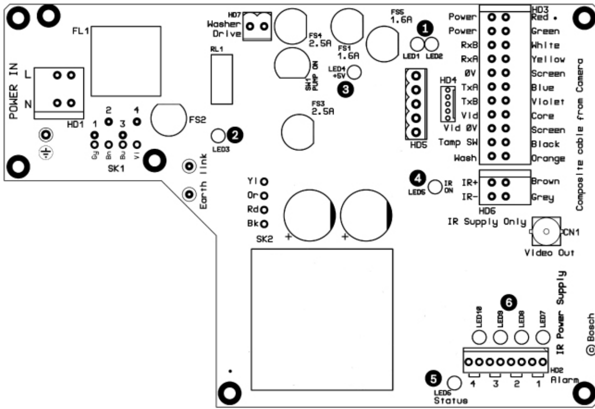
Figure 9.8: Position of LEDs - MIC Series IR power supply PCB
