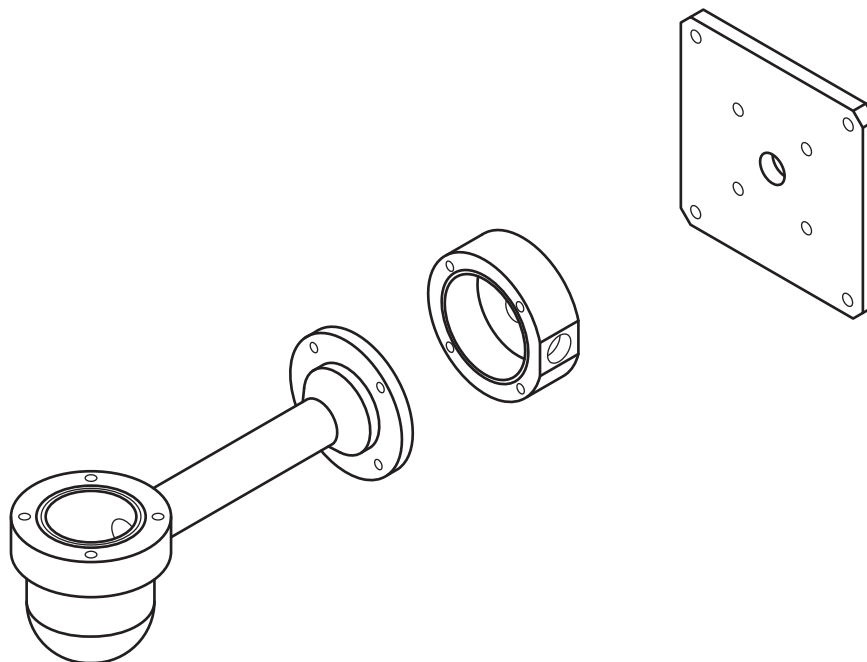
Figure 5.2: Typical wall mount (from left: Wall Mount Bracket (MIC-WMB), Shallow Conduit Adapter (MIC-SCA), and Spreader Plate (MIC-SPR))
