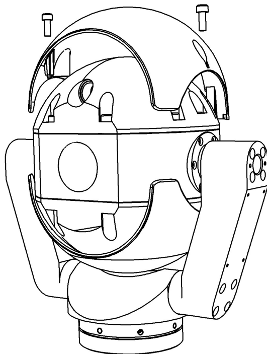
Figure 10.1: Sunshield and Screws being placed
