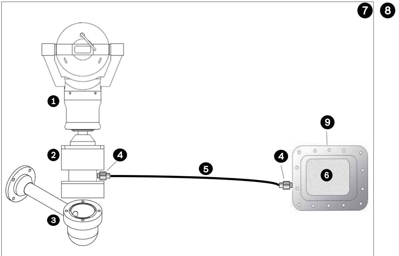
Figure 4.2: Installation of MIC PSU in Hazardous Area
