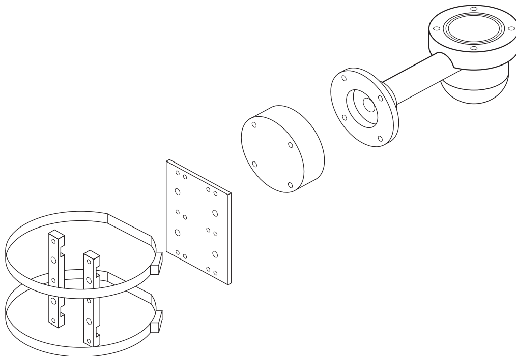
Figure 5.1: Typical pole mount (from left: Pole Mount Bracket (MIC-PMB) [2 mounting blocks, 2 pole bands, and 1 mounting plate], Shallow Conduit Adapter (MIC-SCA), and Wall Mount Bracket (MIC-WMB))
