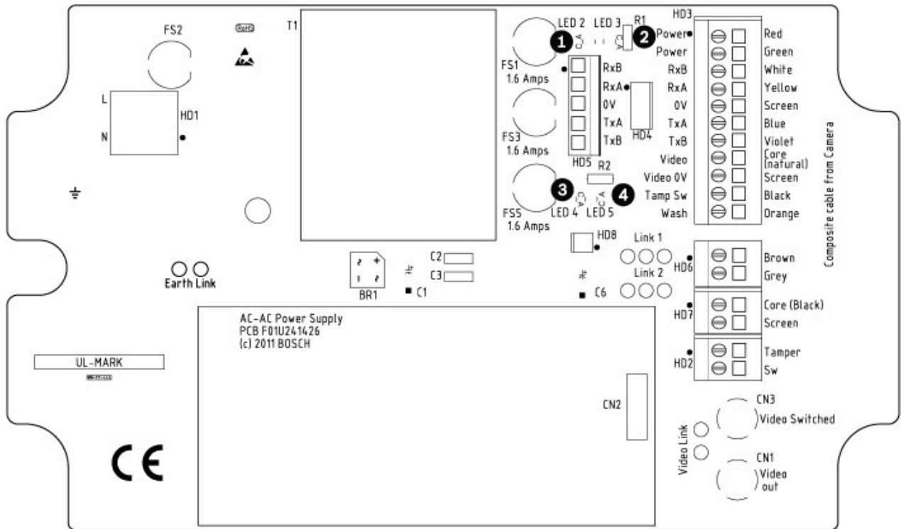
Figure 9.7: Position of LEDs - MIC Series power supply PCB
