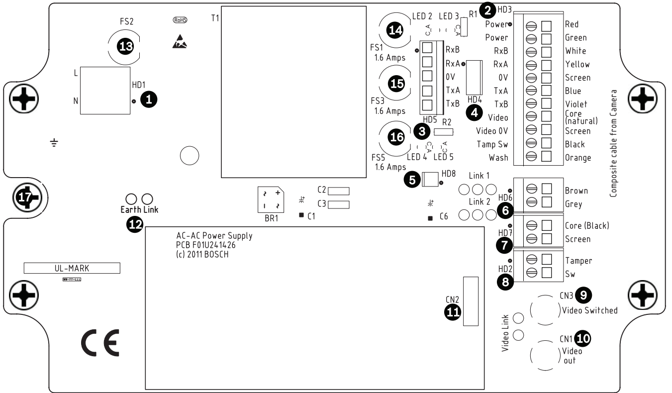
Figure 9.2: Layout of MIC-240PSU-2 and MIC-115PSU-2
