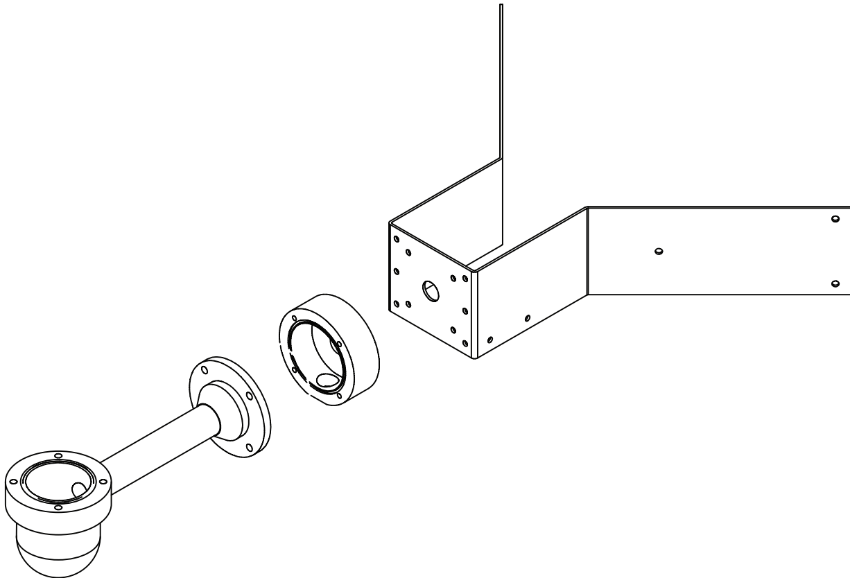
Figure 5.3: Typical corner mount (from left: Wall Mount Bracket (MIC-WMB), Shallow Conduit Adapter (MIC-SCA), and Corner Mount Bracket (MIC-CMB))
