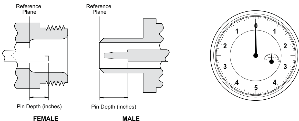
Figure A-1. Pin Depth
