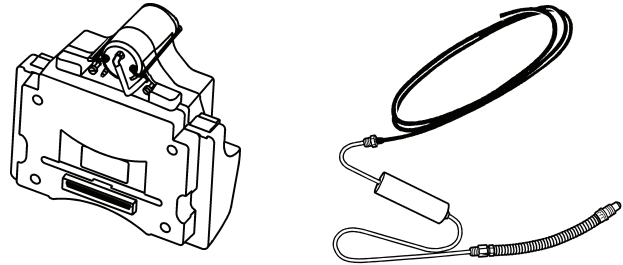
Figure 1.18: Gas M-P Module and Exhaust Test Probe
