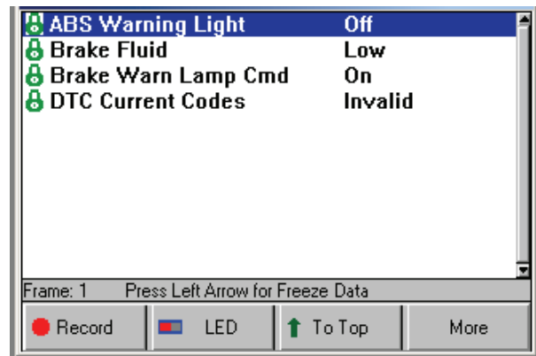
Figure 8.4: Datastream Screen
