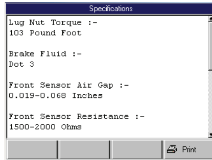
Figure 11.2: Specifications Screen
