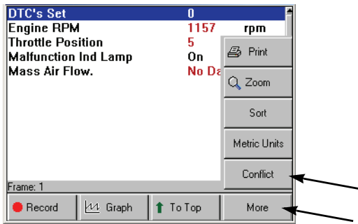
Figure 7.24: More Menu
