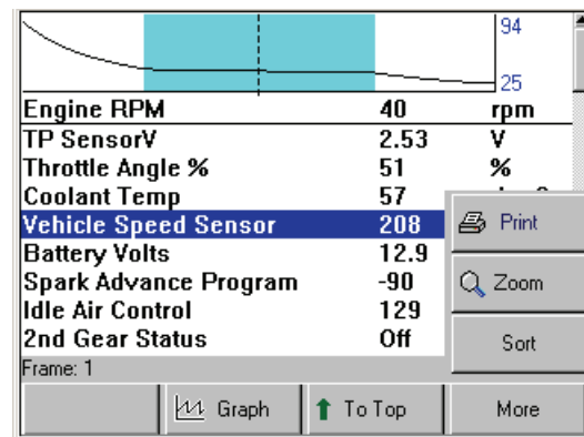
Figure 16.3: Playback Screen
