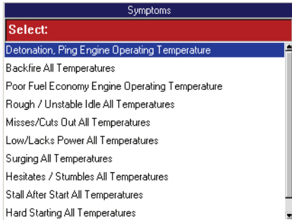
Figure 10.10: Symptoms Screen
