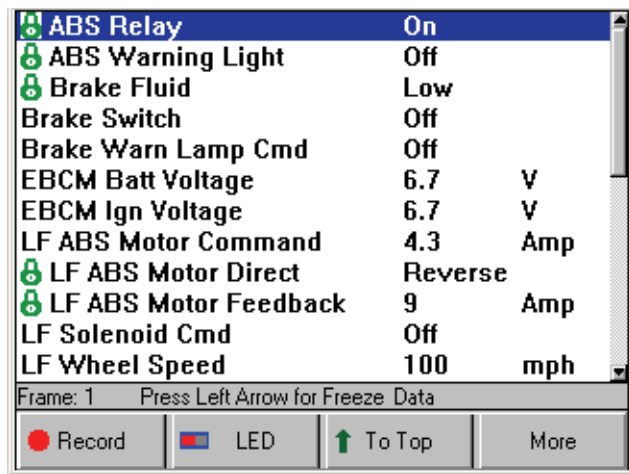
Figure 7.9: Datastream Screen - Sensor Lock Function
