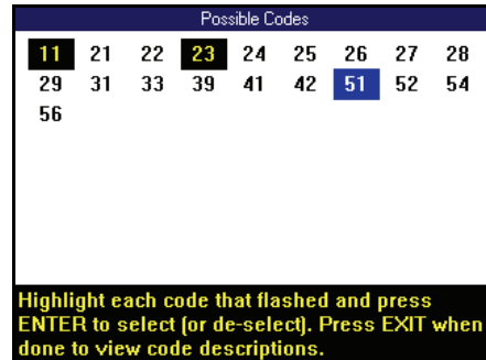
Figure 6.26: Possible Codes Screen
