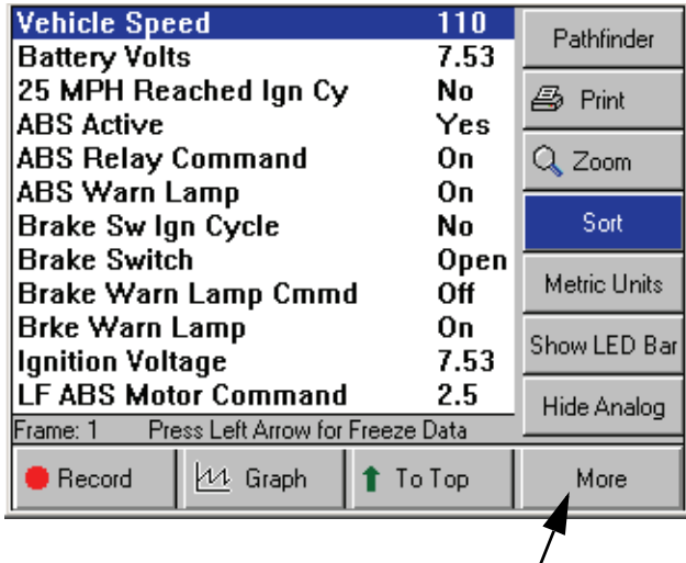
Figure 7.17: Datastream Screen - Sort Function
