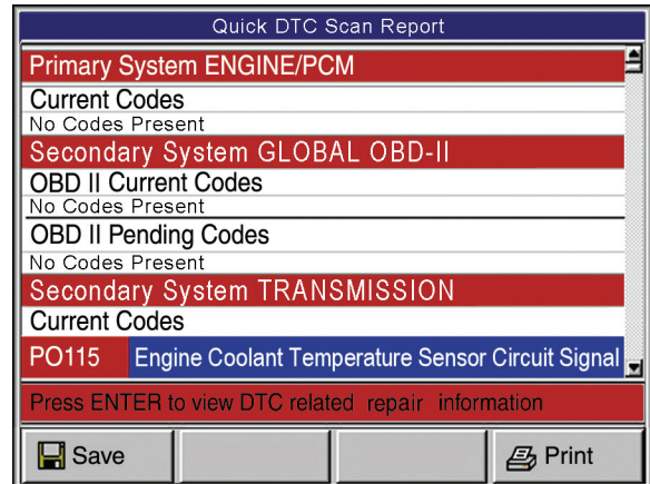
Figure 4.2: Quick DTC Scan Report Screen
