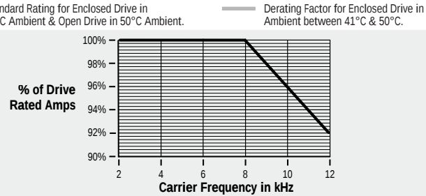
Figure 1 1336E-AQF05-AQF50 and BRF05-BRF100
