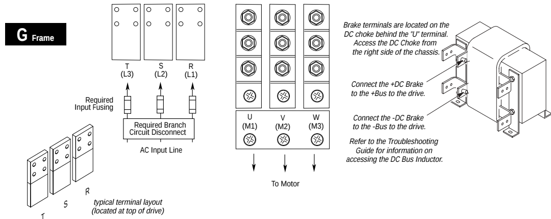
380-480V, 522-597 kW (700-800 HP) Terminal Designations 500-600V, 522-597 kW (700-800 HP) Terminal Designations
