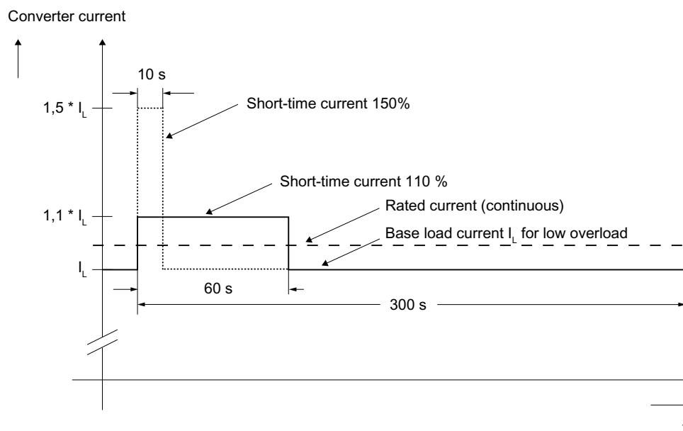
Figure 5-38 Low overload
