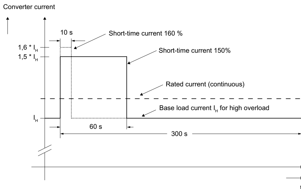
Figure 5-39 High overload
