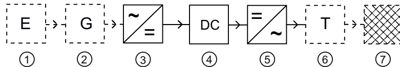
Figure 1-1 Energy flow for power generation with rotating machines
