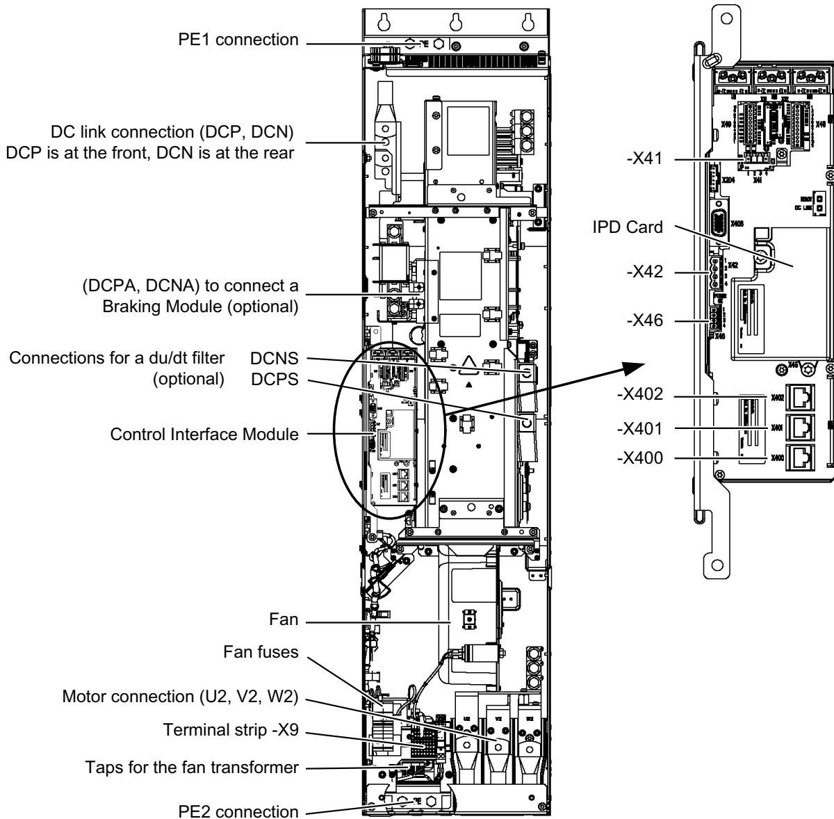
Figure 5-28 Motor Module, frame size FX
