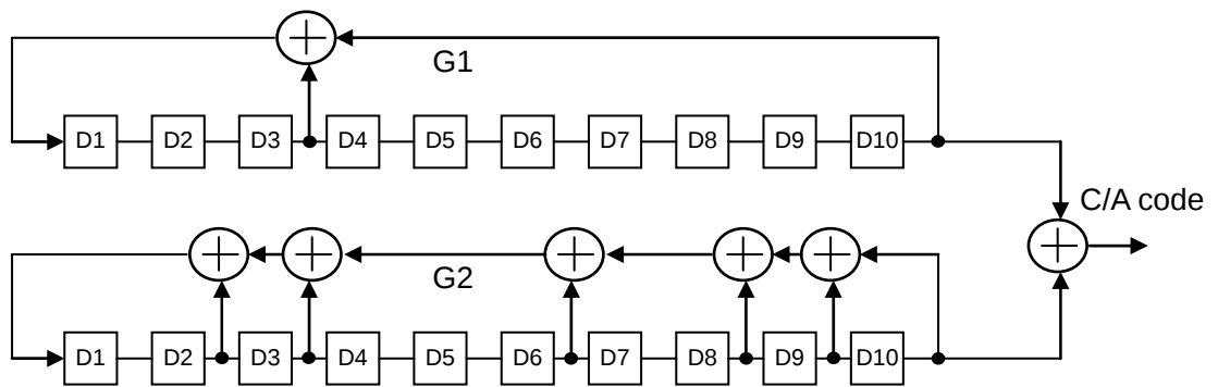
Figure 3.18.1-3 C/A code generation
