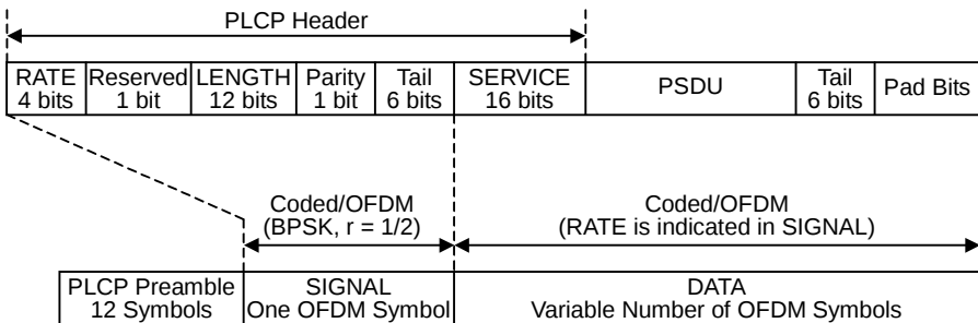
Figure 3.10.1-1 IEEE802.11a PPDU frame format
