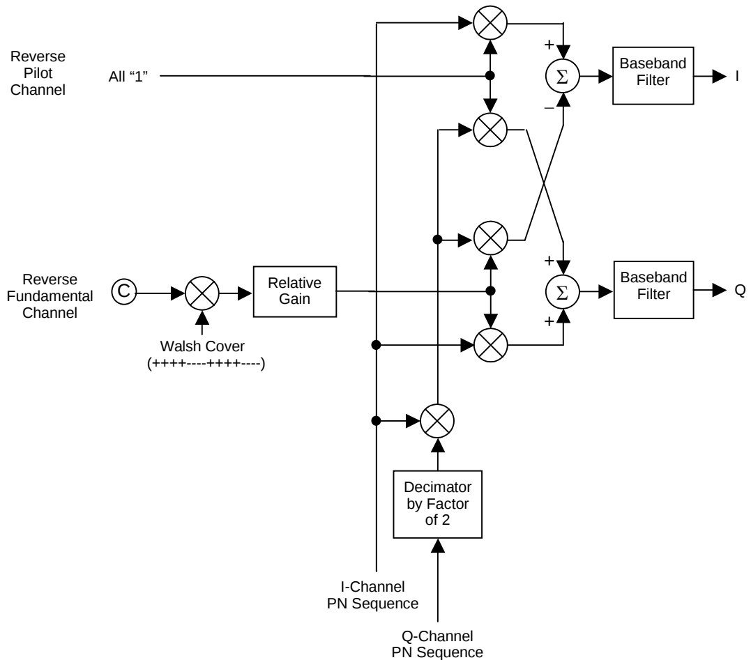
Figure 3.8.6-3 Signal generation block diagram of waveform pattern RVS_RC4_FCH (2/2)
