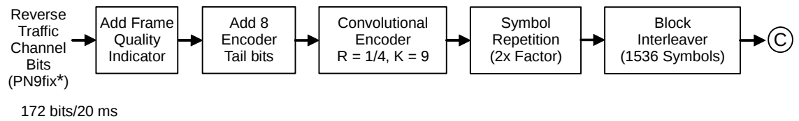
Figure 3.8.4-2 Signal generation block diagram of waveform pattern RVS_RC3_FCH_SCH (1/2)
