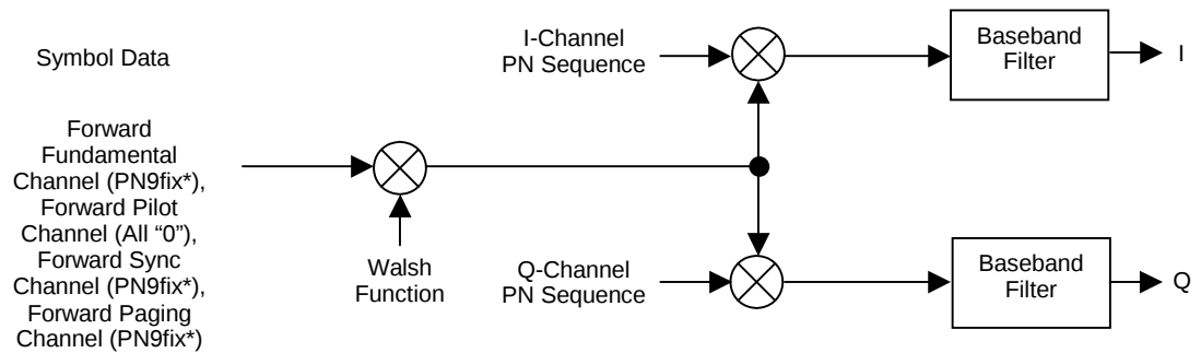
Figure 3.8.7-1 Signal generation block diagram of waveform pattern FWD_RC1-2 9channel
