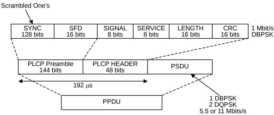
Figure 3.10.2-1 IEEE802.11b Long PLCP PPDU frame format
