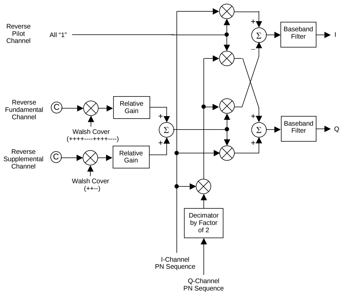
Figure 3.8.4-3 Signal generation block diagram of waveform pattern RVS_RC3_FCH_SCH (2/2)
