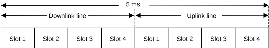
Figure 3.6.1-1 PHS frame configuration
