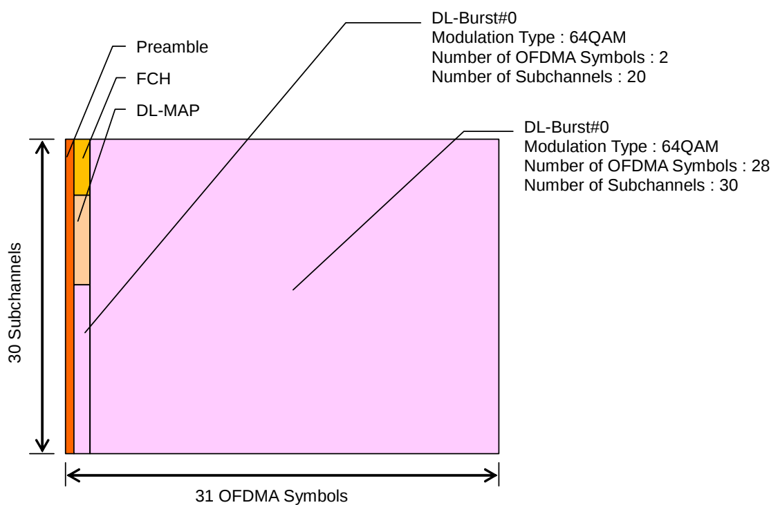
Figure 3.14.1-2 WiMAX_DL_10MHz_64QAM Frame Composition
