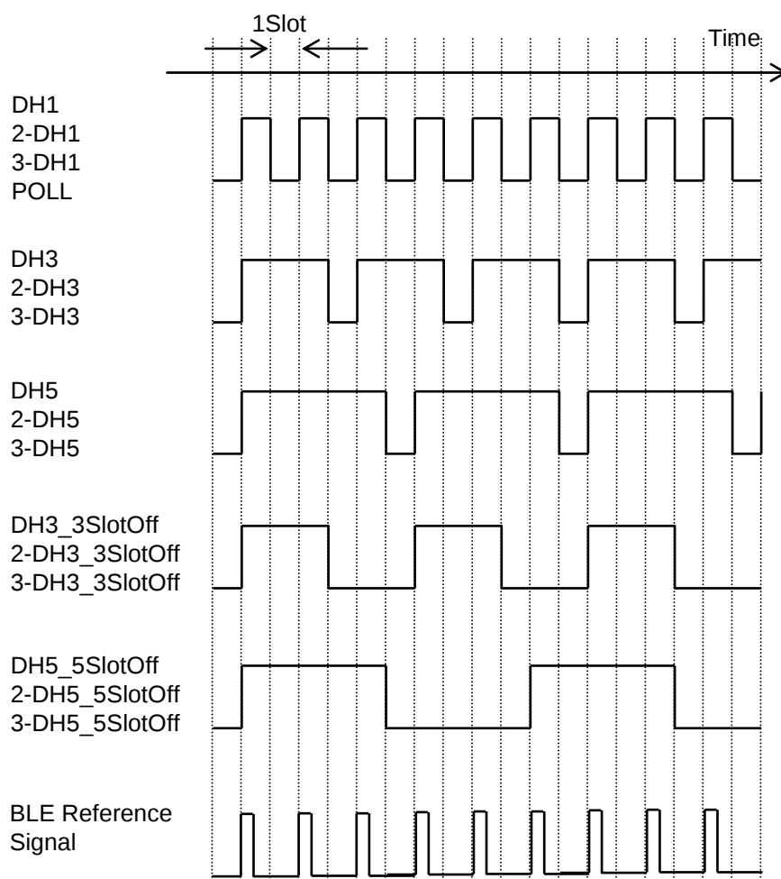
Figure 3.12-1 Timing chart of waveform patterns
