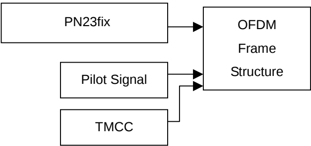
Figure 3.11.1-2 Generation of the waveform patterns for ISDB-T
