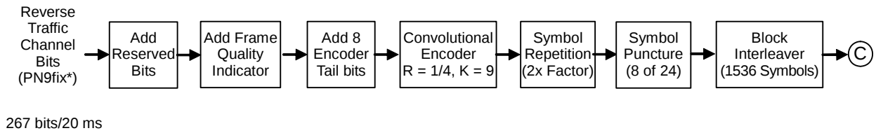
Figure 3.8.6-2 Signal generation block diagram of waveform pattern RVS_RC4_FCH (1/2)
