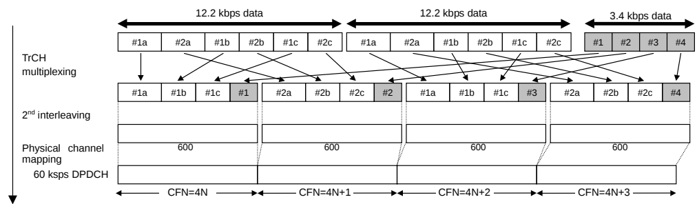
Figure 3.1.2-2 Channel coding and multiplexing for UL AMR TFCSx (2 of 2)
