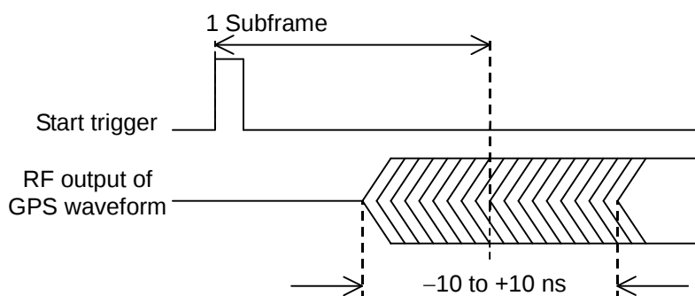
Figure 3.13-1 SYNC_ADJ output timing
