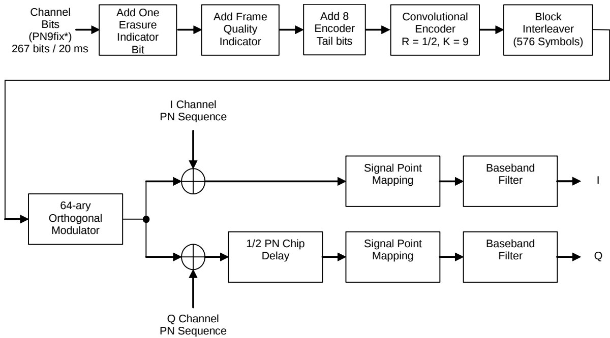
Figure 3.8.2-2 Signal generation block diagram of waveform pattern RVS_RC2_FCH
