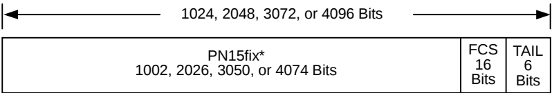
Figure 3.9.1-1 Format of 1xEV-DO forward packet
