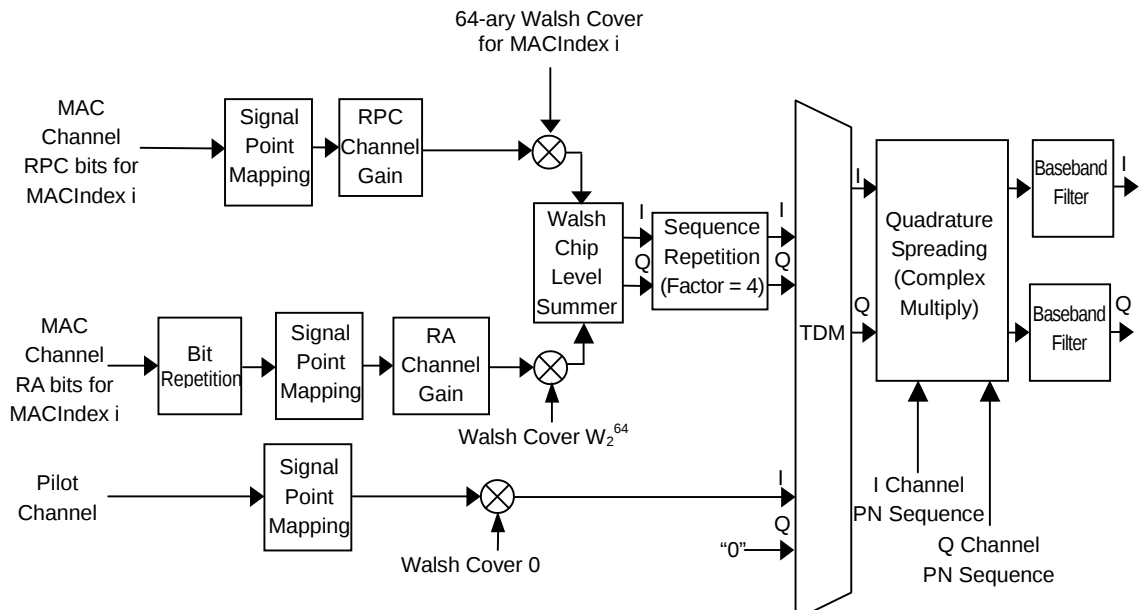
Figure 3.9.3-1 Signal generation block diagram of 1xEV-DO forward idle slot waveform pattern
