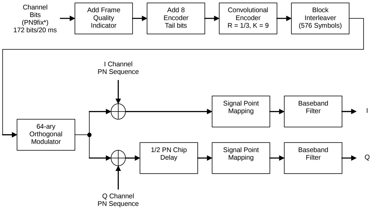
Figure 3.8.1-2 Signal generation block diagram of waveform pattern RVS_RC1_FCH
