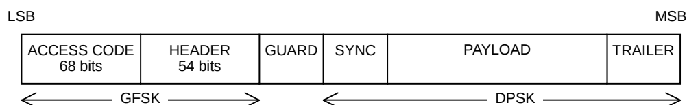
Figure 3.12.2-1 Packet configuration for Enhanced Data Rate waveform
