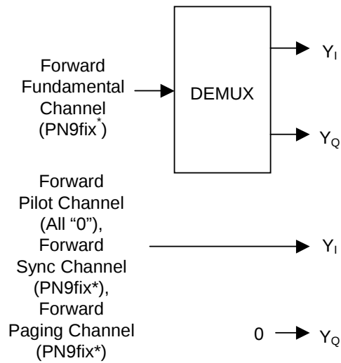
Figure 3.8.8-1 Signal generation block diagram of waveform pattern FWD_RC3-5 9channel (1/2)
