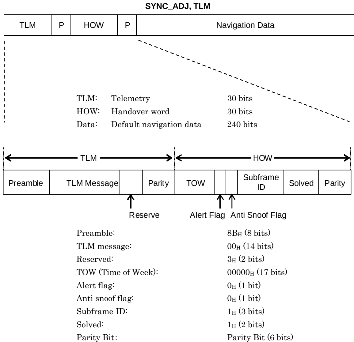
Figure 3.13.1-1 Waveform format of GPS
