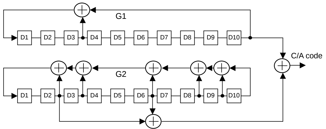
Figure 3.13.1-4 C/A code generation
