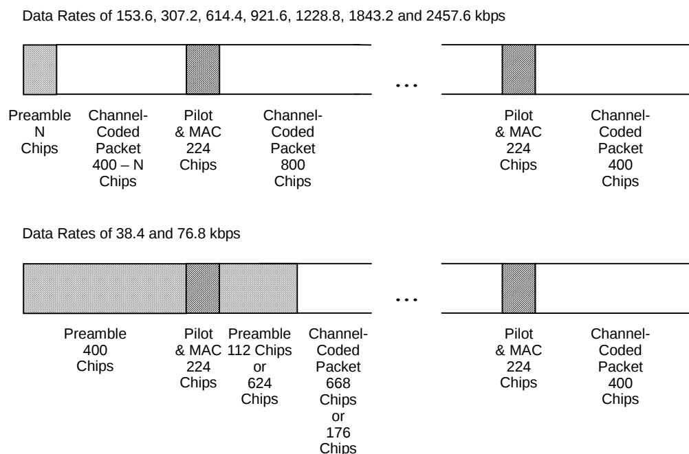
Figure 3.9.1-4 TDM timing diagram
