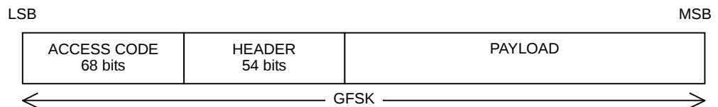
Figure 3.12.1-1 Packet configuration for Basic Rate waveform
