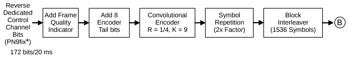
Figure 3.8.5-2 Signal generation block diagram of waveform pattern RVS_RC3_DCCH (1/2)
