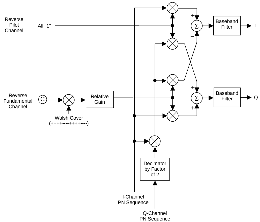
Figure 3.8.3-3 Signal generation block diagram of waveform pattern RVS_RC3_FCH (2/2)
