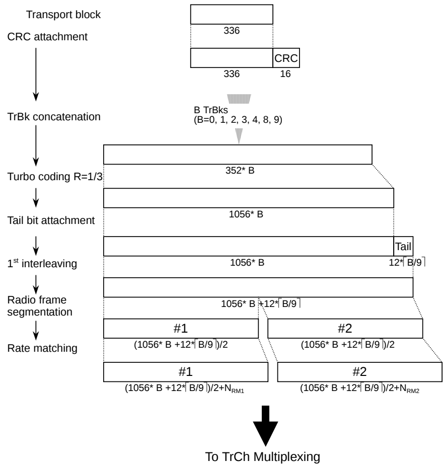
Figure 3.1.2-5 Channel coding for UL 64 kbps packet
