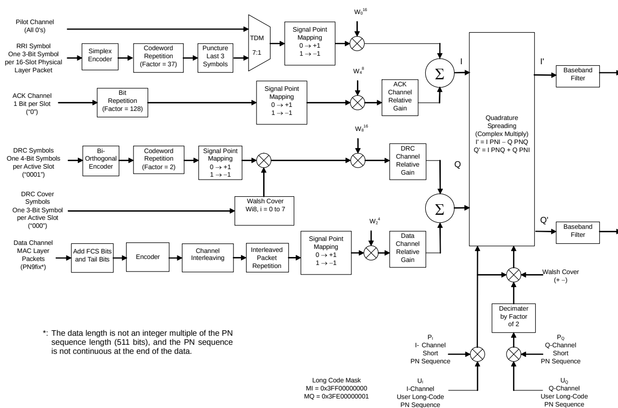
Figure 3.9.2-2 Signal generation block diagram of 1xEV-DO reverse waveform pattern
