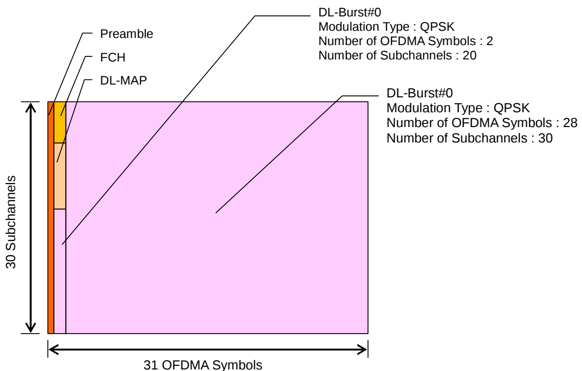
Figure 3.14.1-1 WiMAX_DL_10MHz_QPSK Frame Composition
