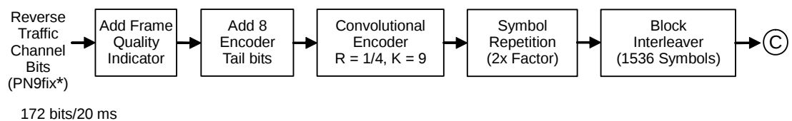
Figure 3.8.3-2 Signal generation block diagram of waveform pattern RVS_RC3_FCH (1/2)
