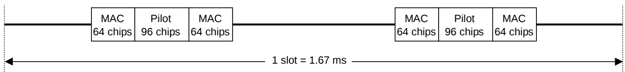
Figure 3.9.3-2 Format of 1xEV-DO forward idle slot waveform pattern
