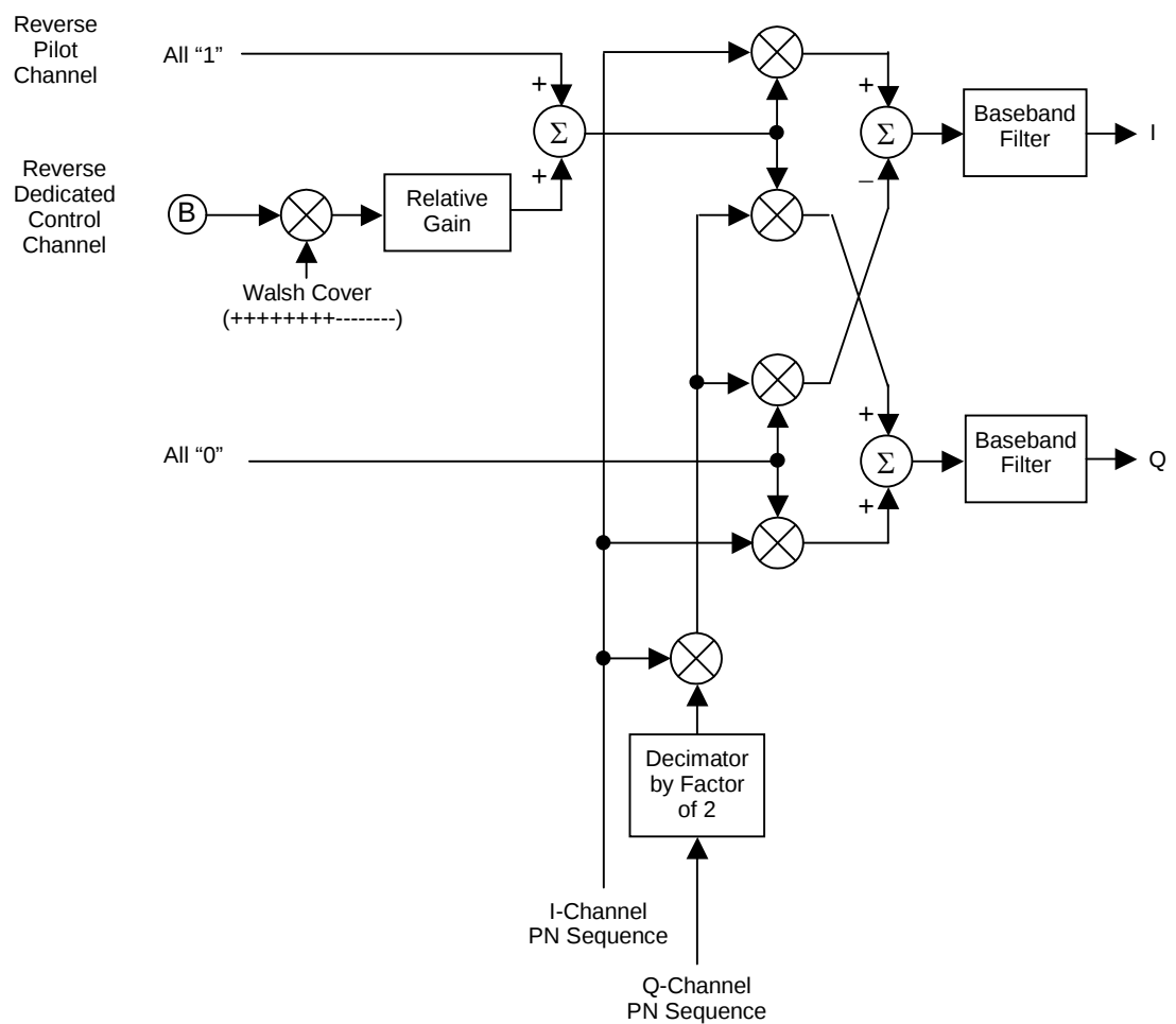
Figure 3.8.5-3 Signal generation block diagram of waveform pattern RVS_RC3_DCCH (2/2)
