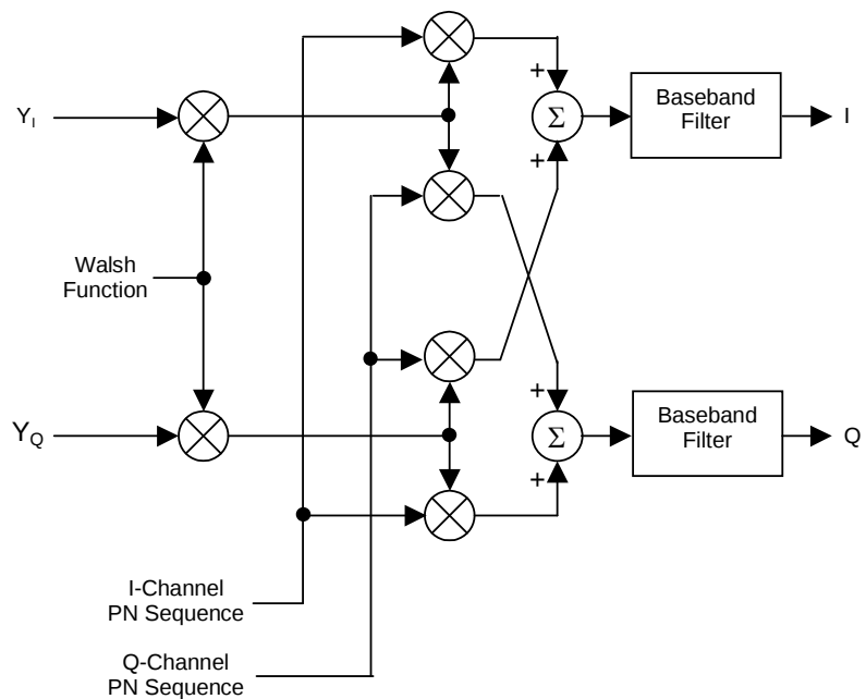
Figure 3.8.8-2 Signal generation block diagram of waveform pattern FWD_RC3-5 9channel (2/2)
