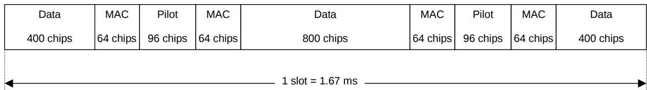
Figure 3.9.1-3 Slot format of 1xEV-DO forward waveform pattern (excluding idle slot)
