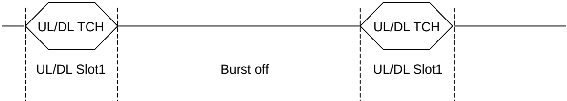
Figure 3.6.1-2 Output of waveform pattern other than PI_4_DQPSK_PN9/15/ALL0
