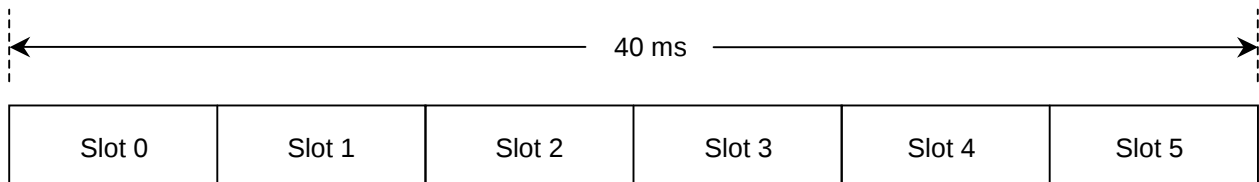
Figure 3.4.1-2 Frame configuration at half rate
