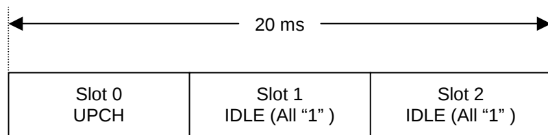
Downlink UPCH 1-slot transmission (DL_Packet_Slot_0)
