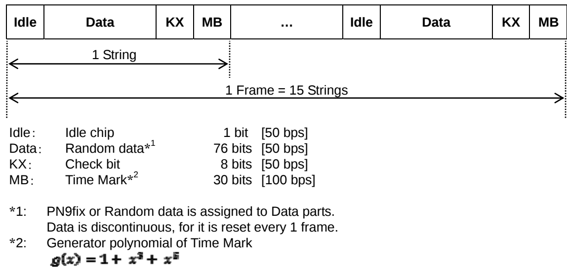
Figure 3.17.1-1 Waveform format of 15String_PN9 and 15String_Message
