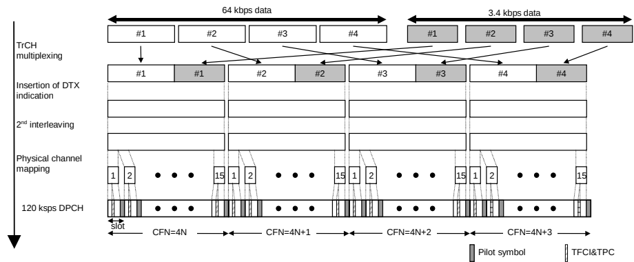
Figure 3.1.5-3 Channel coding and multiplexing for DL ISDN
