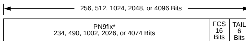
Figure 3.9.2-1 Format of 1xEV-DO reverse packet
