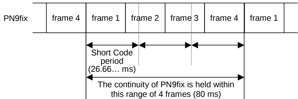
Figure 3.8.1-3 PN9fix data and short code
