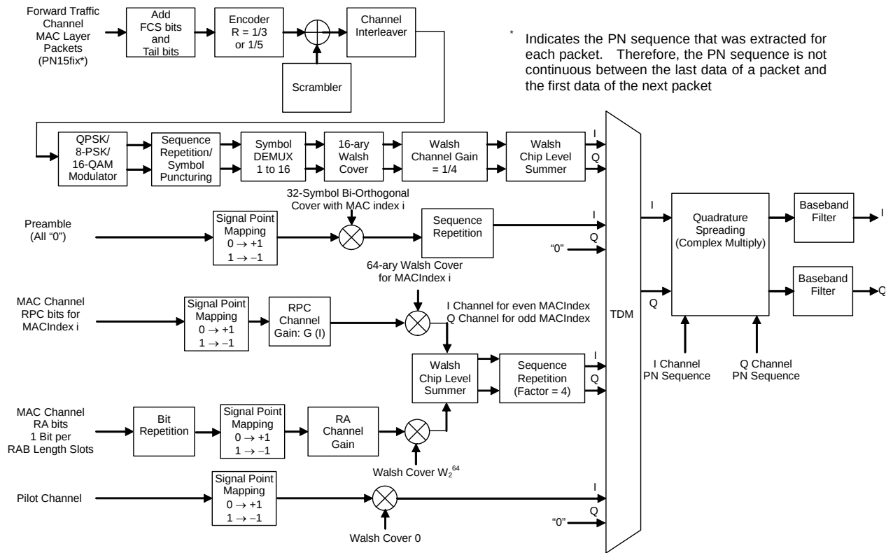
Figure 3.9.1-2 Signal generation block diagram of 1xEV-DO forward waveform pattern
