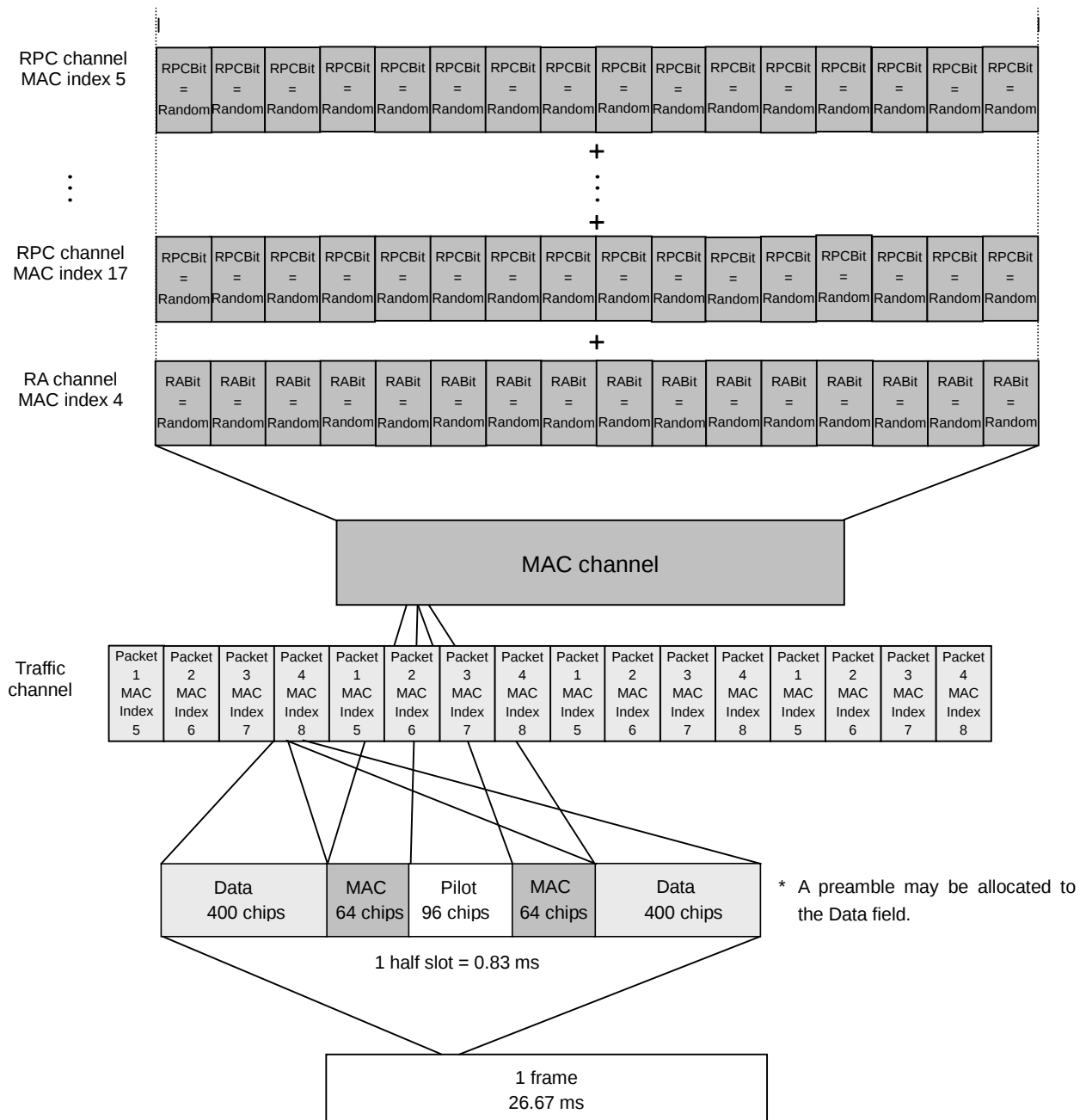
Figure 3.9.1-5 Multiplexing channels
