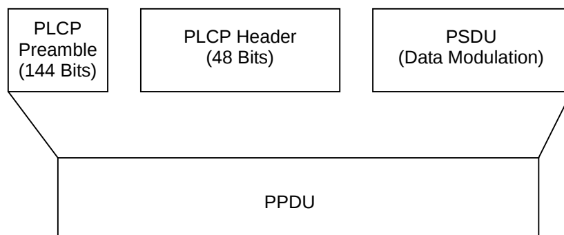
Figure 3.10.3-1 IEEE802.11b Long preamble PPDU frame format
