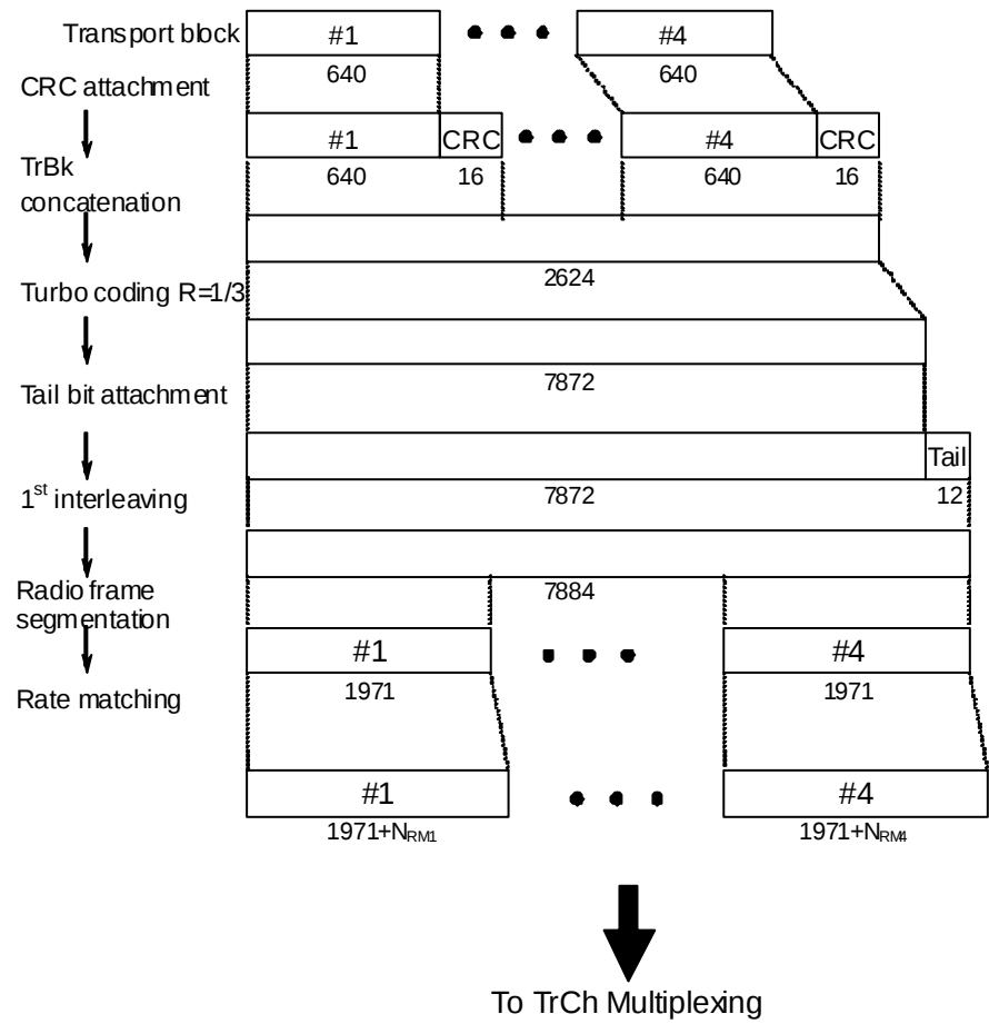
Figure 3.1.2-3 Channel coding for UL ISDN
