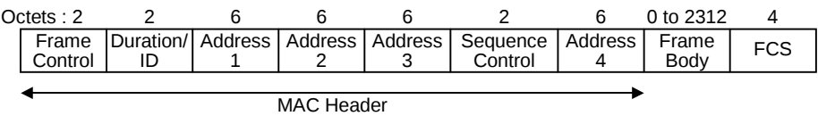
Figure 3.10.1-2 IEEE802.11a MAC frame format
