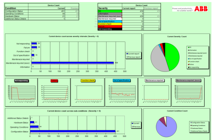
Figure 12: Process instruments report
