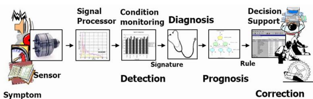
Figure 4: Predictive maintenance control loop model
