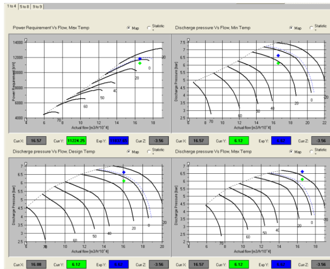
Figure 11: Compressor asset monitoring
