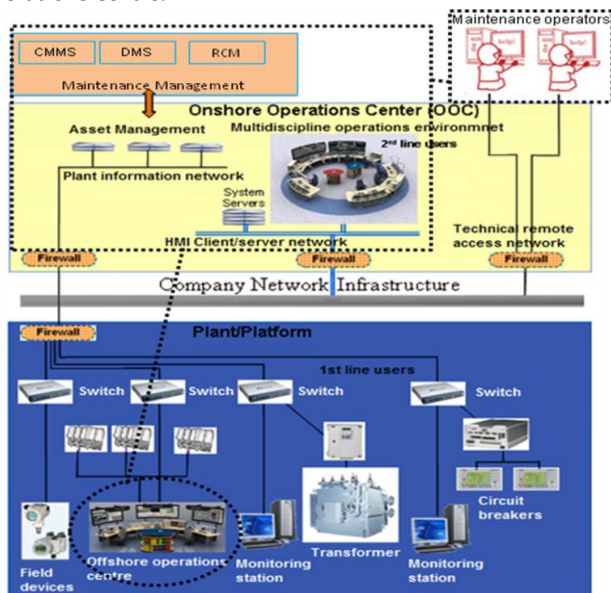
Figure 7: AO topology shown in dotted lines
