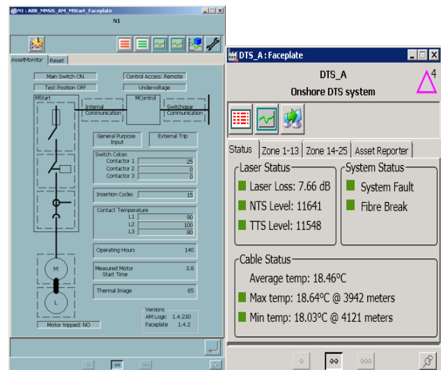
Figure 10: Contactor and DTS asset monitoring faceplates
