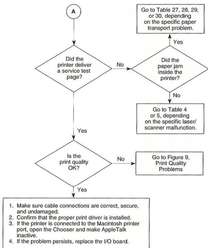
Flowchart 2 LaserWriter Select 300 Print Engine Error (2 of 2)
