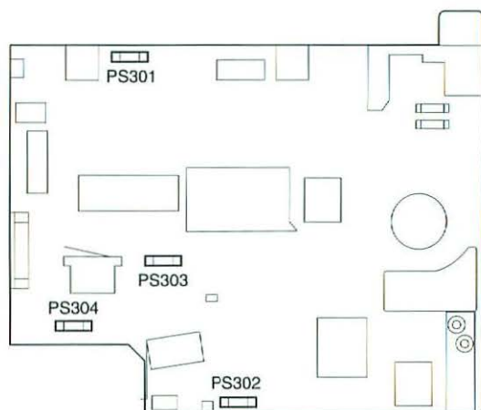
Figure 7 Sensing System
