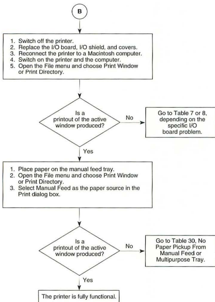
Flowchart 4 LaserWriter Select 310 Print Engine Error (3 of 3)
