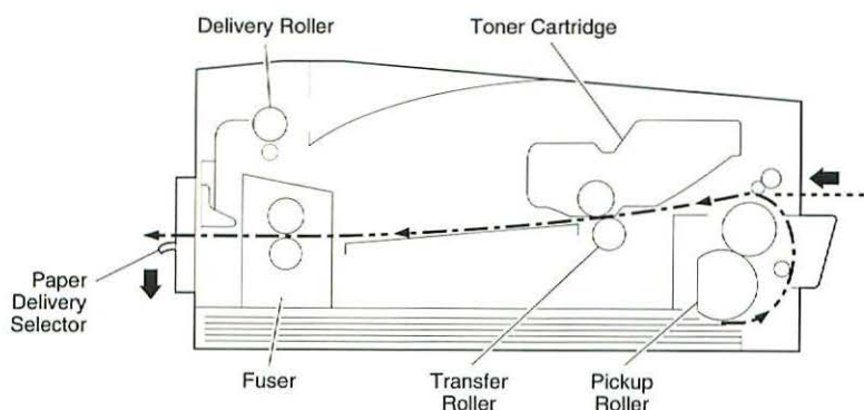
Figure 5 Face-Up Path
