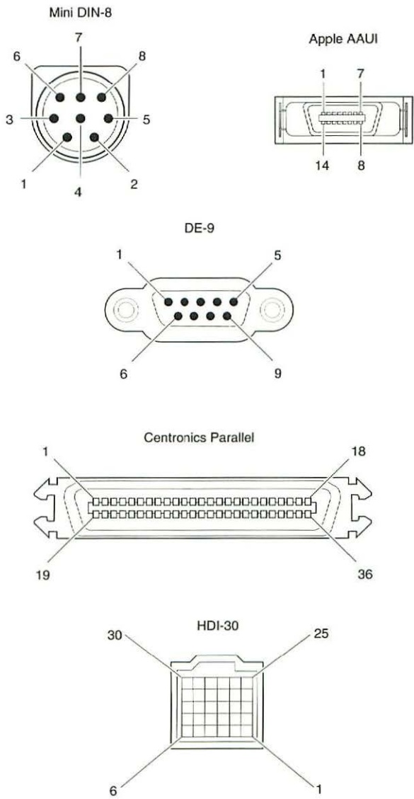
Figure 3 Cable Connectors
