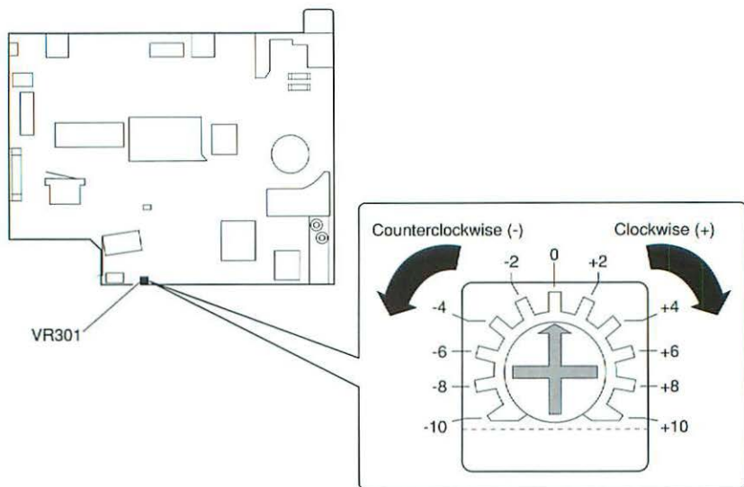
Figure 15 Resetting VR301
