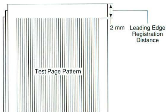
Figure 14 Optimum Registration
