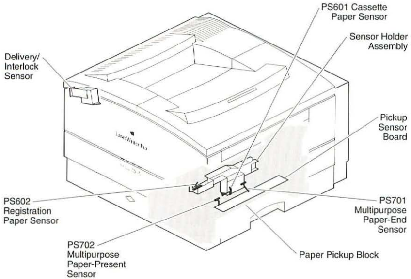
Figure 11 Sensing System
