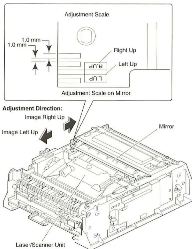
Figure 13 Readjusting the Mirror Alignment
