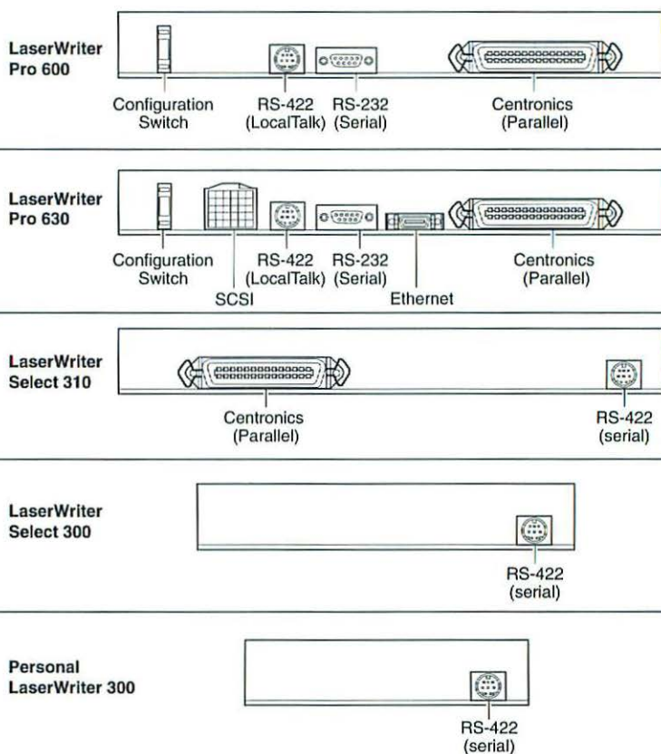
Figure 4 External Connectors on the Printers
