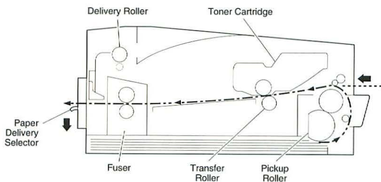
Figure 6 Face-Down Path
