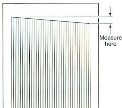
Figure 12 Measuring the Adjustment Error
