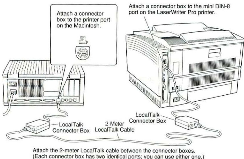
Figure 1 LocalTalk Connection
