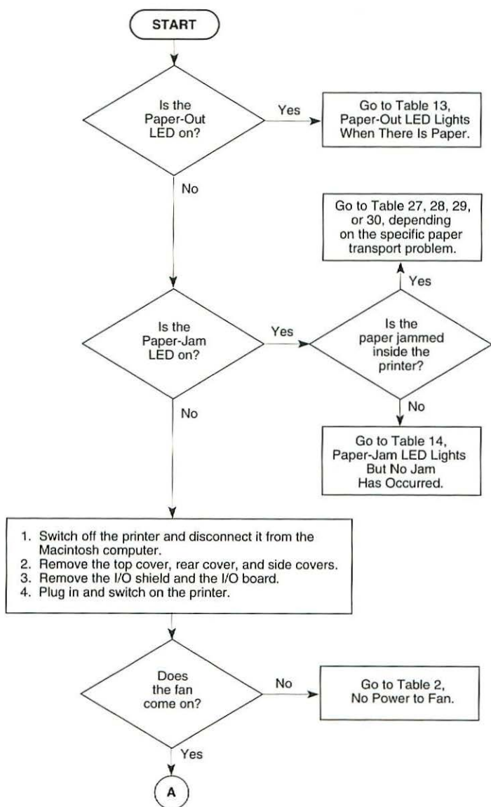
Flowchart 4 LaserWriter Select 310 Print Engine Error (1 of 3)
