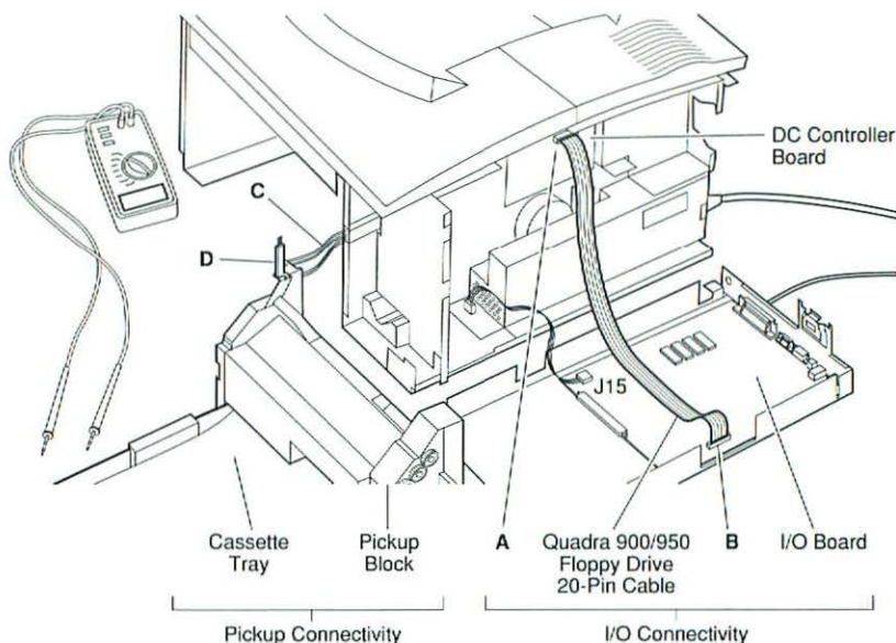
Figure 9 Maintaining Connectivity
