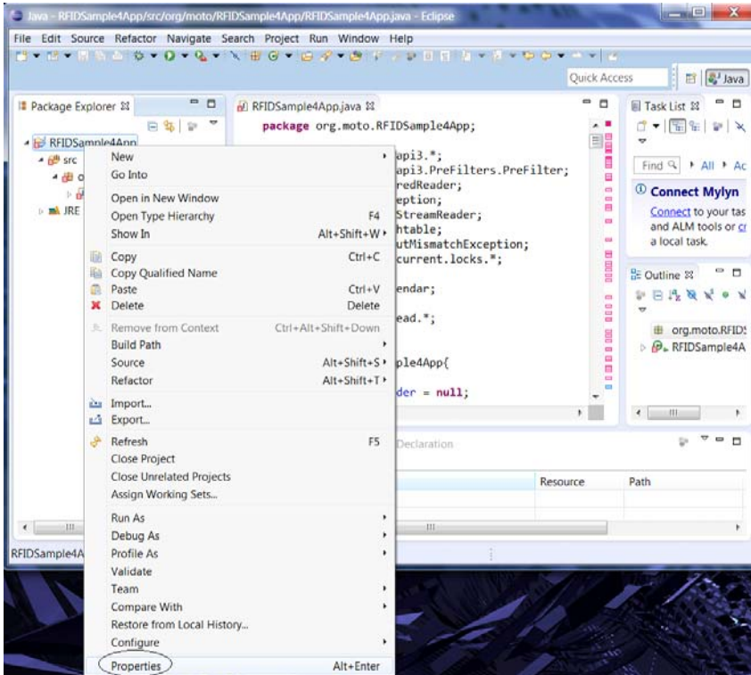
Figure 20 Selecting Properties
