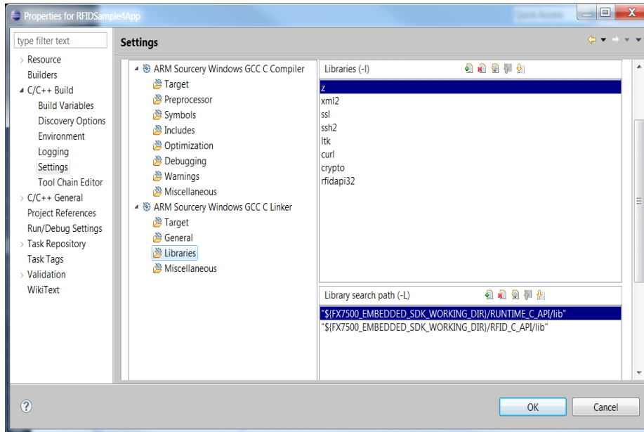
Figure 69 Linker Libraries
