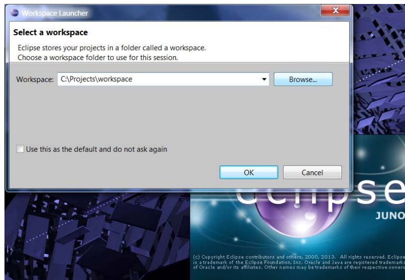
Figure 1 Workspace Window
