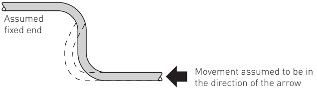
Figure B2: Two right angle bends
