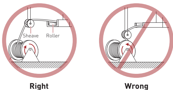
Figure 7: Reel setup
