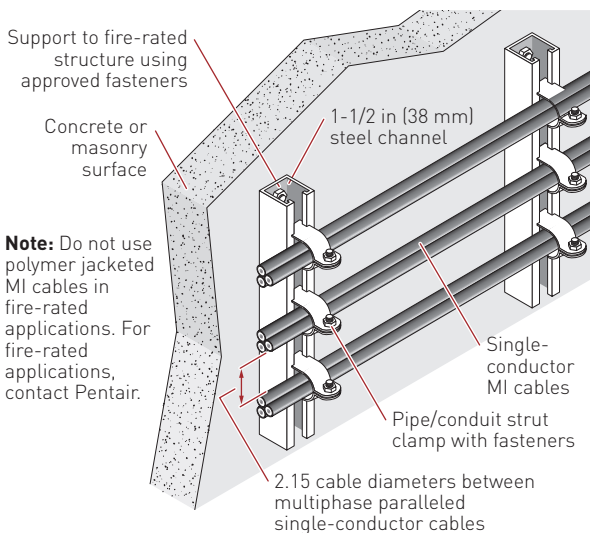
Figure 3: Pipe clamp
