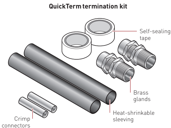
Figure 34: System 1850 termination kits
