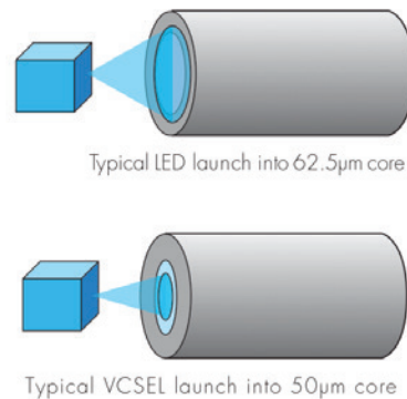
Figure 1 - Overfilling LED and under-filling VCSEL launches
