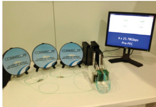
Figure 9 - 4 x 25 Gb/s WDM over 225 m of LazrSPEED 550 WideBand MMF at OFC 2015
