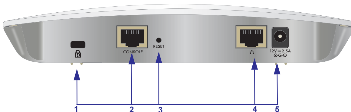
Figure 2. Rear panel
