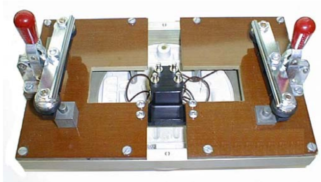
Figure 255 –Form 2K Meter Test Adapter #9707-8009, to test meter in socket type test board
