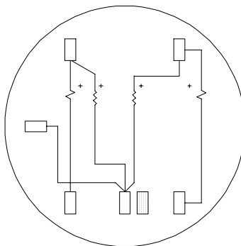
– Form 25S (Network)
