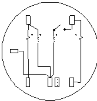
Figure 13 – Form 12S (Network)
