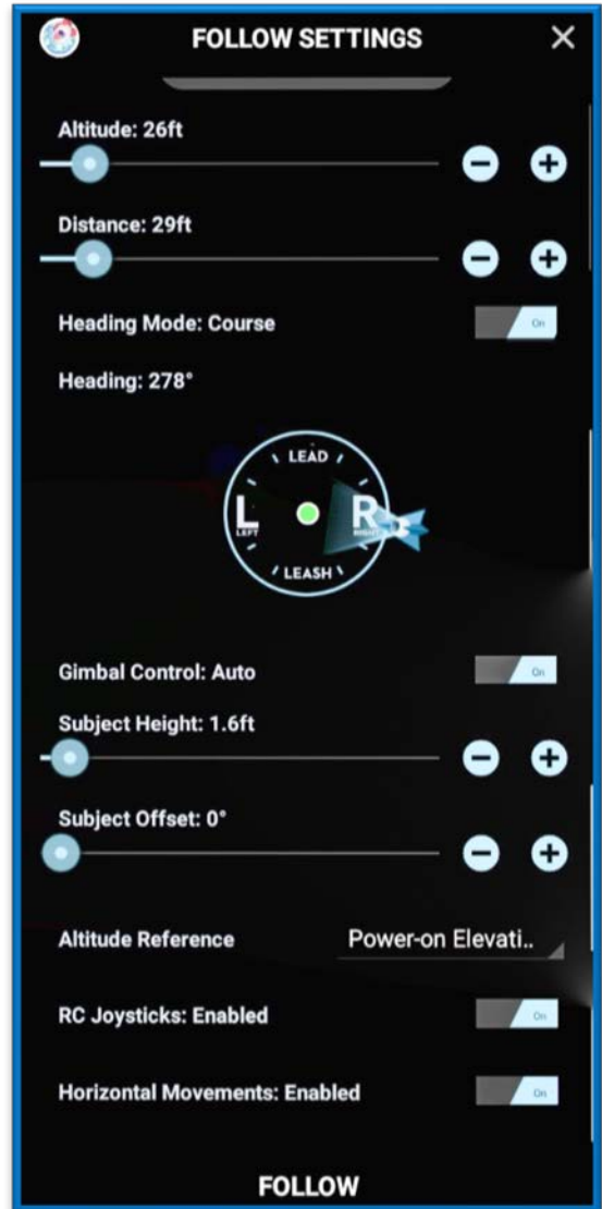
Figure 38 - Follow Mode Settings
