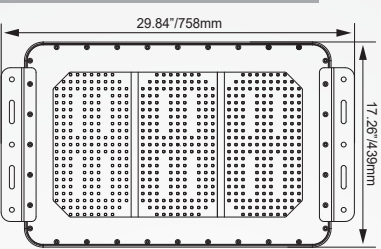
3-DIGIT 2D VIEW
