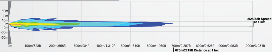
XPR-27M | 9891682 - Tilted Beam
