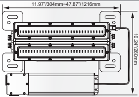
ITEM #: CSWD192PE Shown PART #: 9893105
