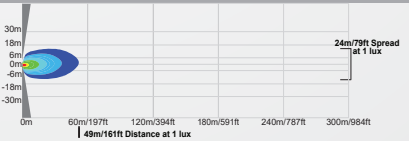
XIL-201 | 4007468 - FLOOD BEAM
