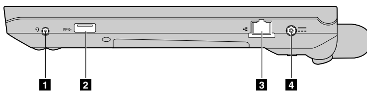
Figure 5. Lenovo ZhaoYang K29 right-side view
