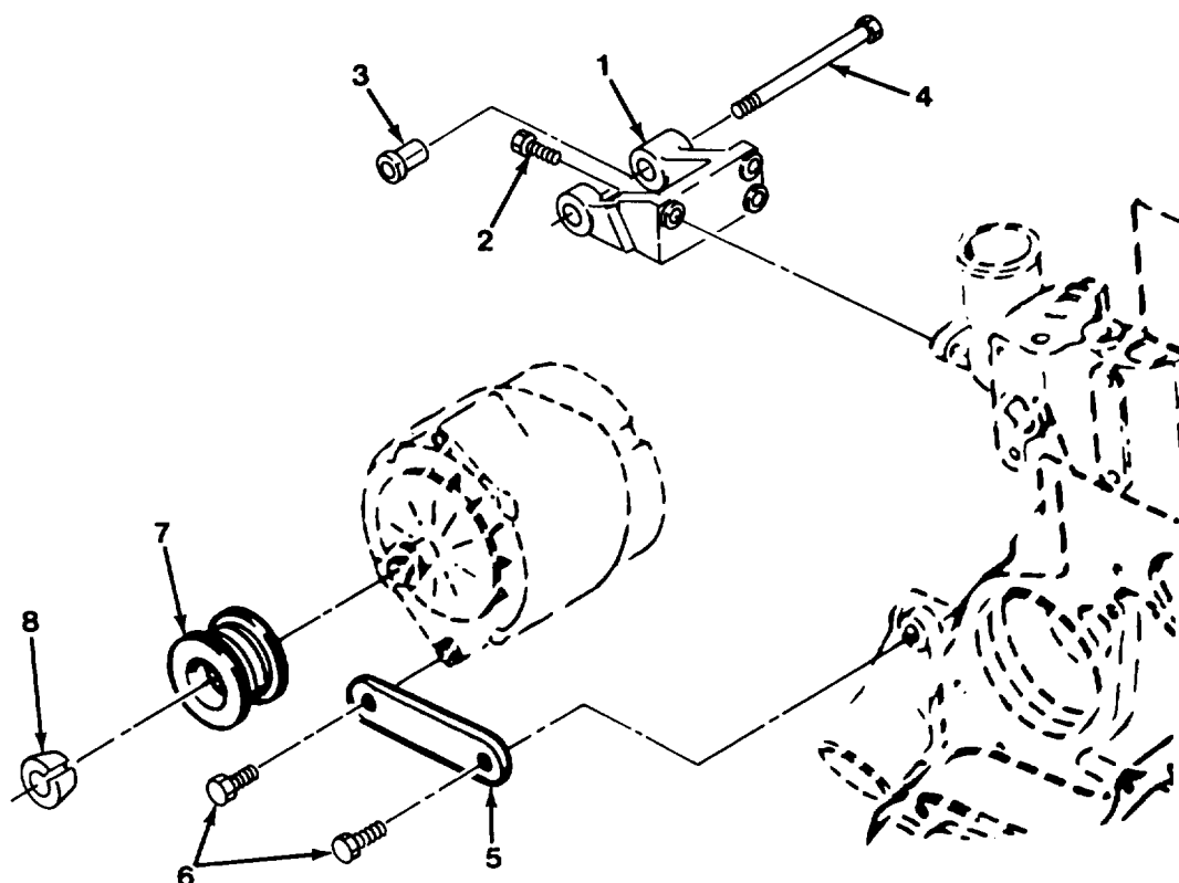
Figure 6-3. Alternator Mounting.
