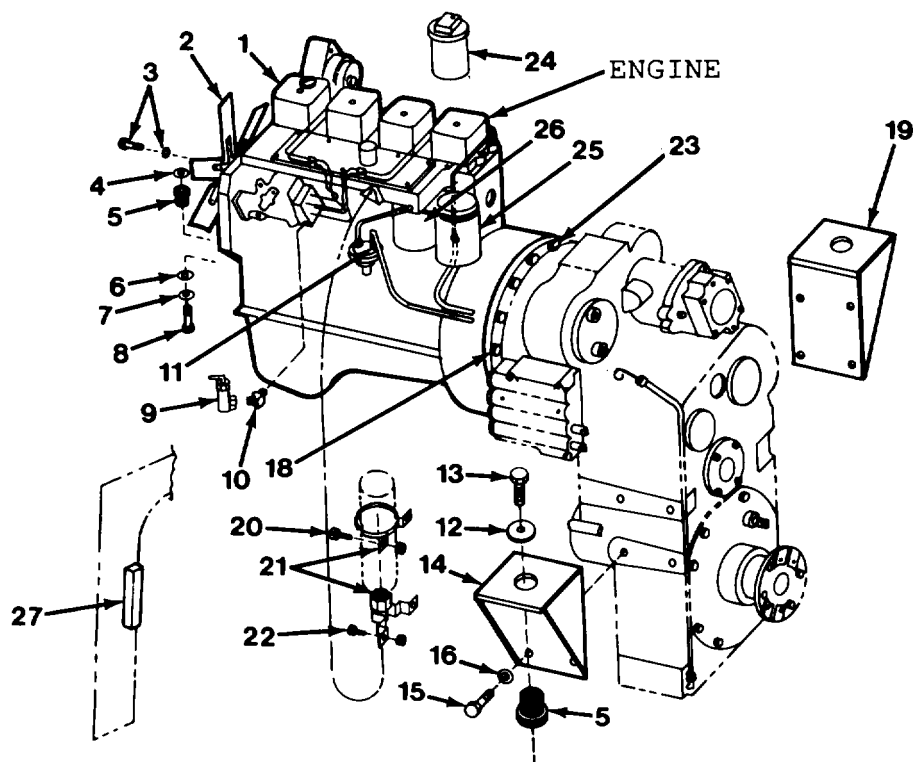
Figure 2-1.Engine Assembly
