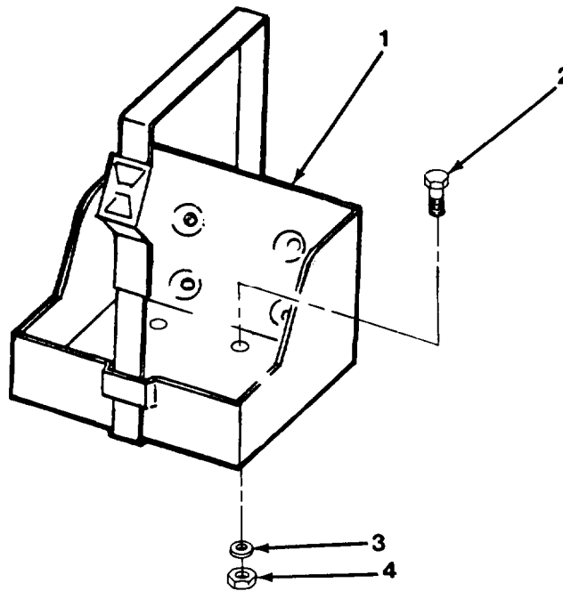
Figure 11-3. Can Bracket.
