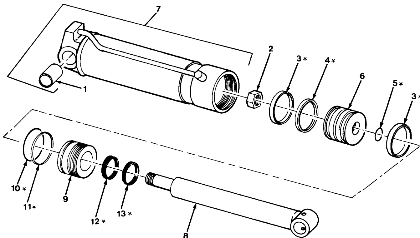
Figure 10-5. Outrigger Cylinder.
