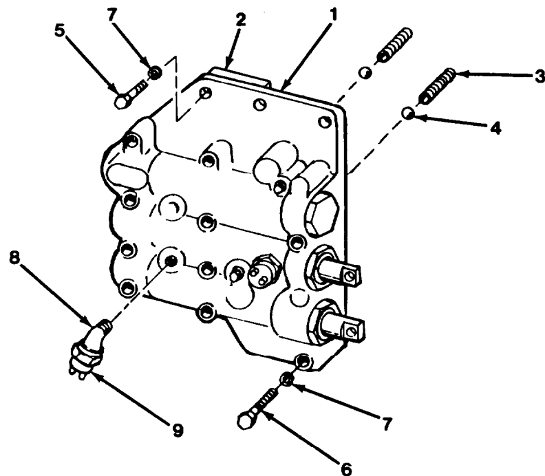
Figure 7-7, Valve Group
