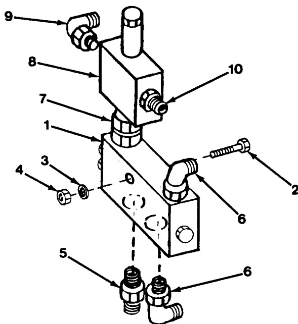
Figure 10-27. Steering Valve Fittings.
