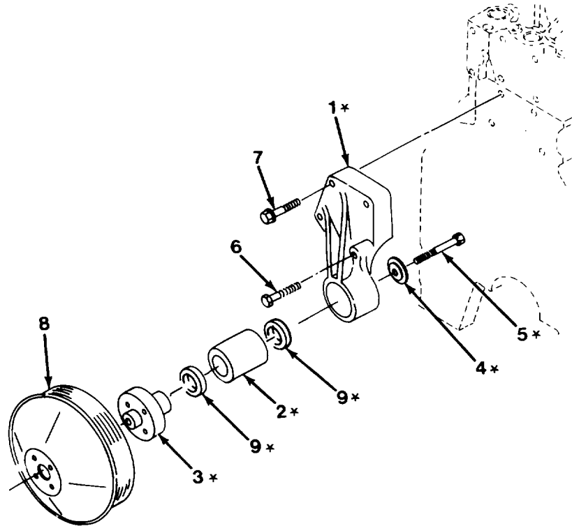
Figure 5-4. Fan Support.
