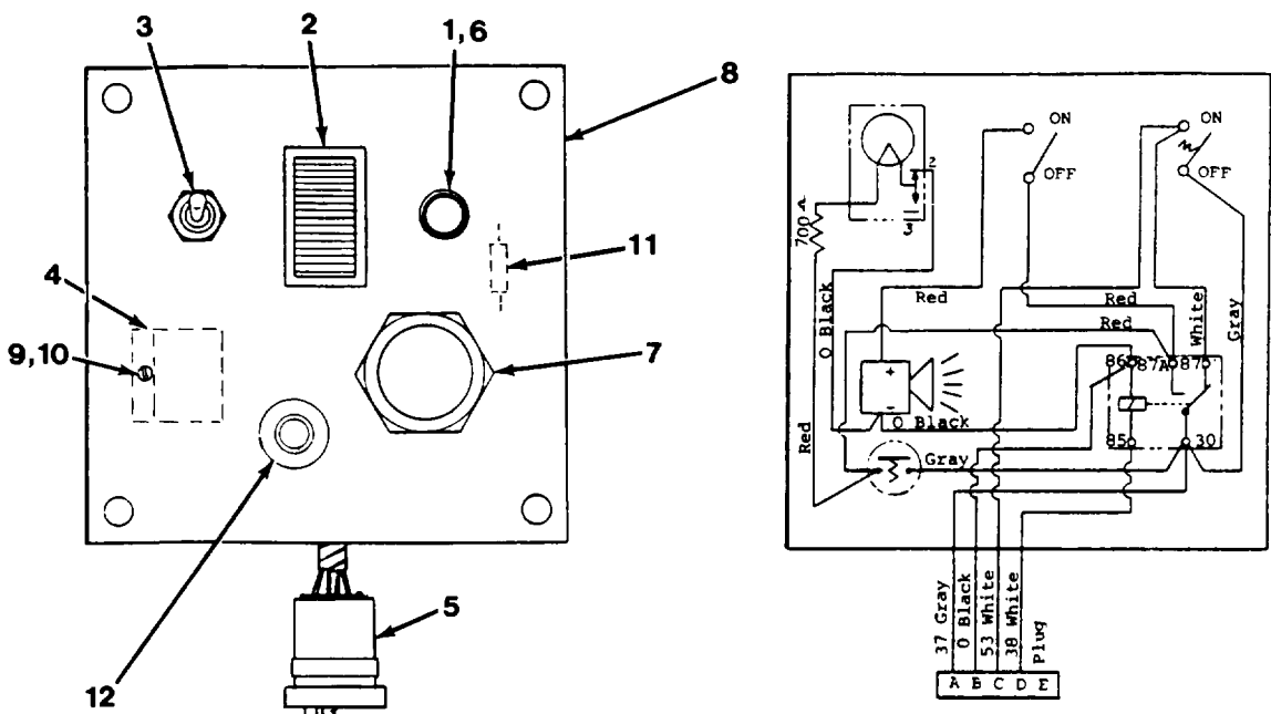
Figure 6-12. Anti-Two Block Control Panel.
