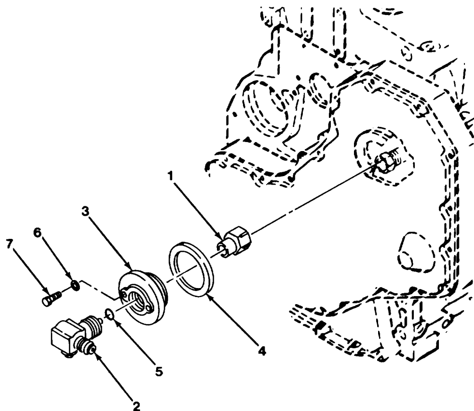
Figure 2-17. Front Gear Train Accessory Drive.
