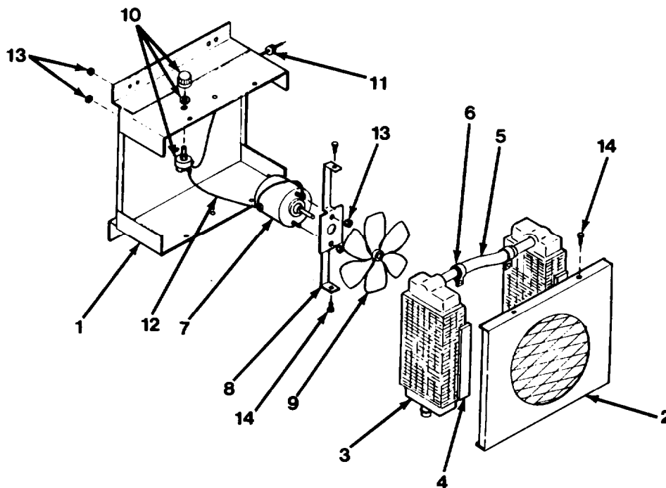
Figure 14-9. Heater.
