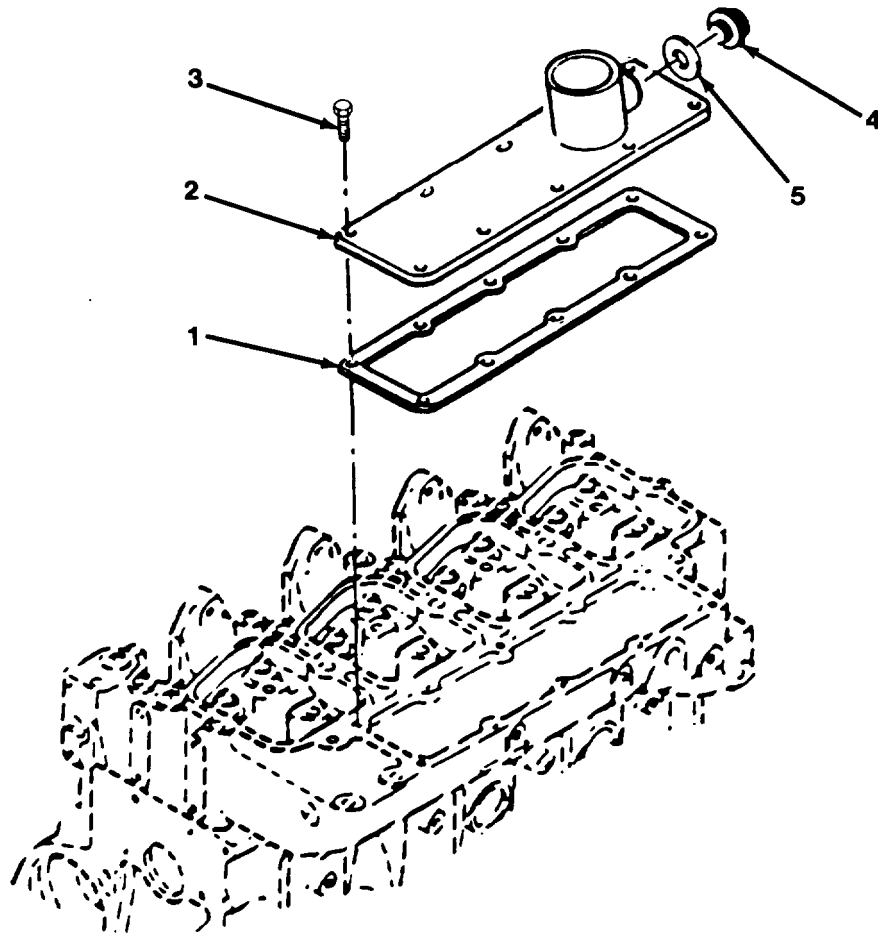
Figure 2-25. Air Intake Manifold.
