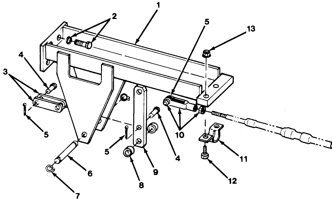
Figure 7-9 Transmission Control.
