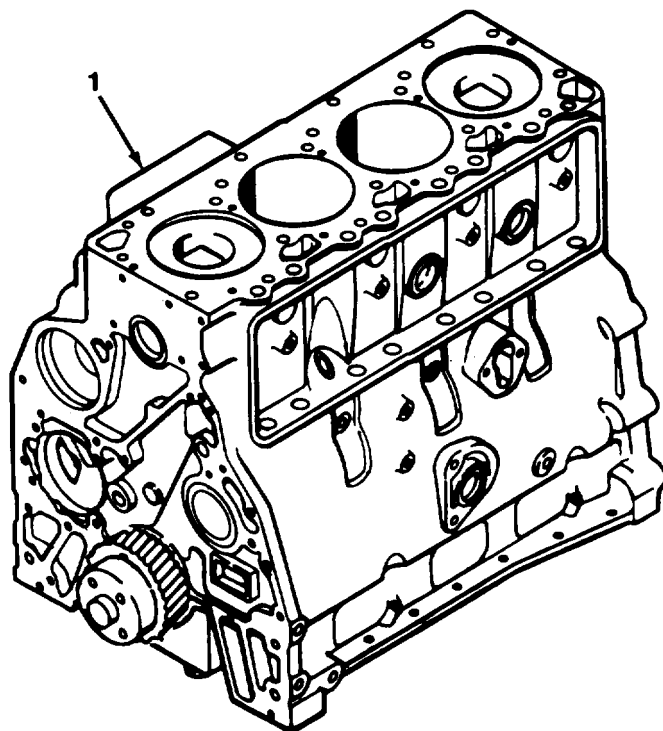
Figure 2-3. Short Block
