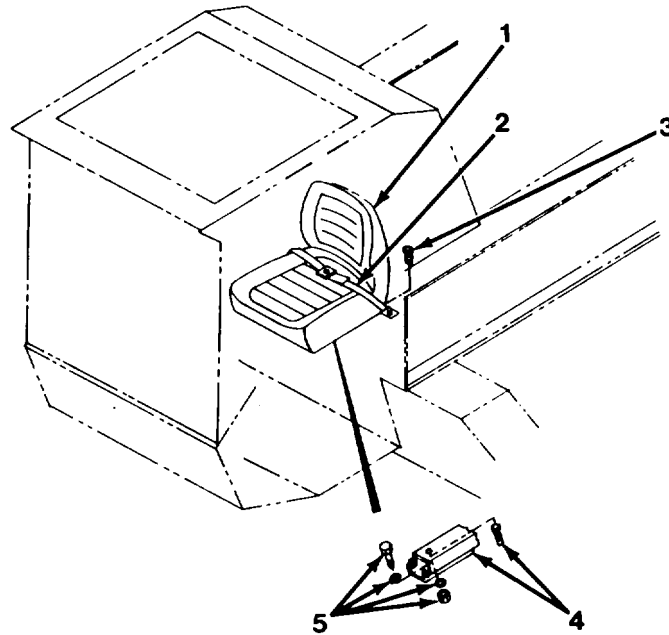
Figure 11-11. Seat
