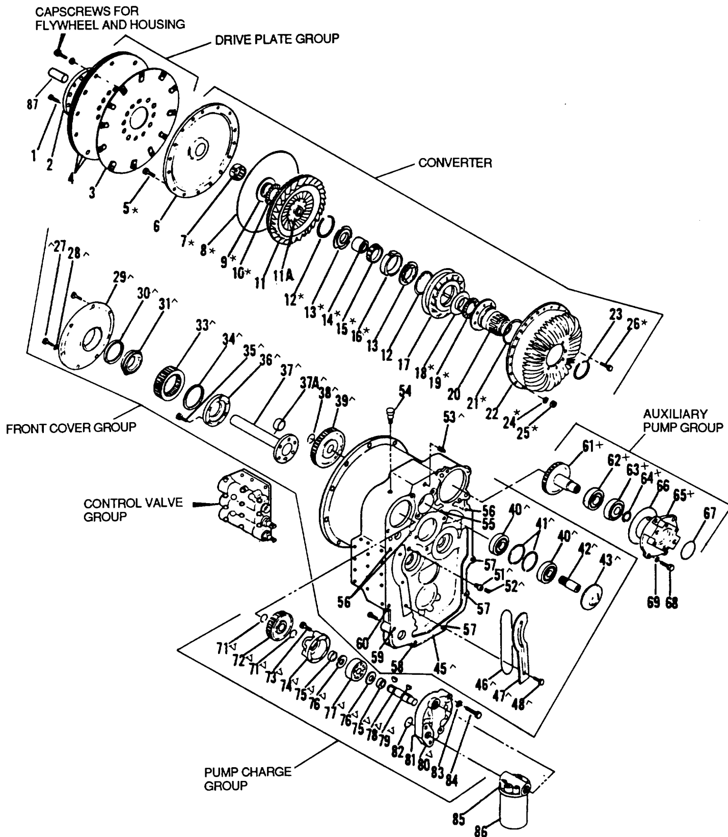
Figure 7-2. Transmission Assembly - 1.
