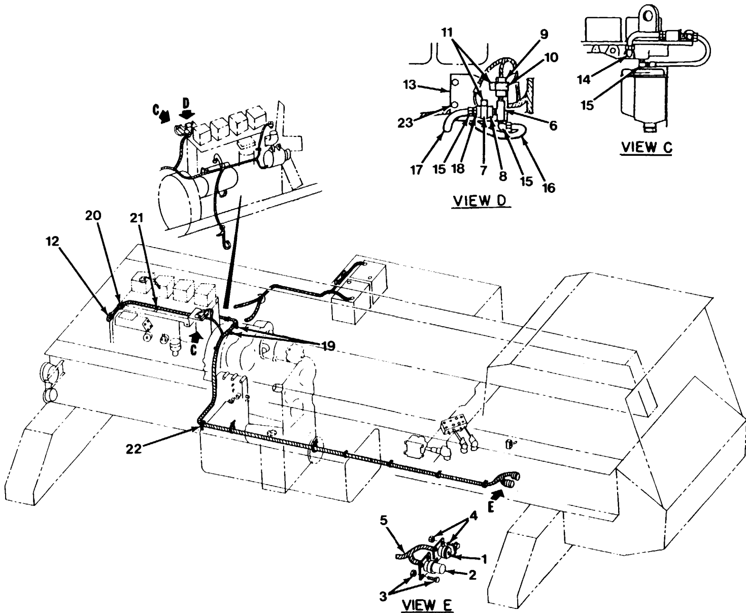
Figure 6-15. SIE-ICE Electrical System
