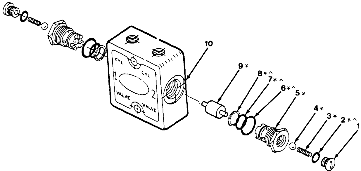
Figure 10-6. Outrigger Hold Valve.
