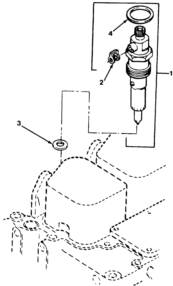
Figure 3-4 . Fuel Injector
