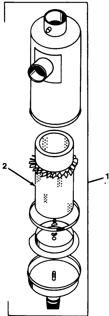
Figure 2-24. Air Cleaner.
