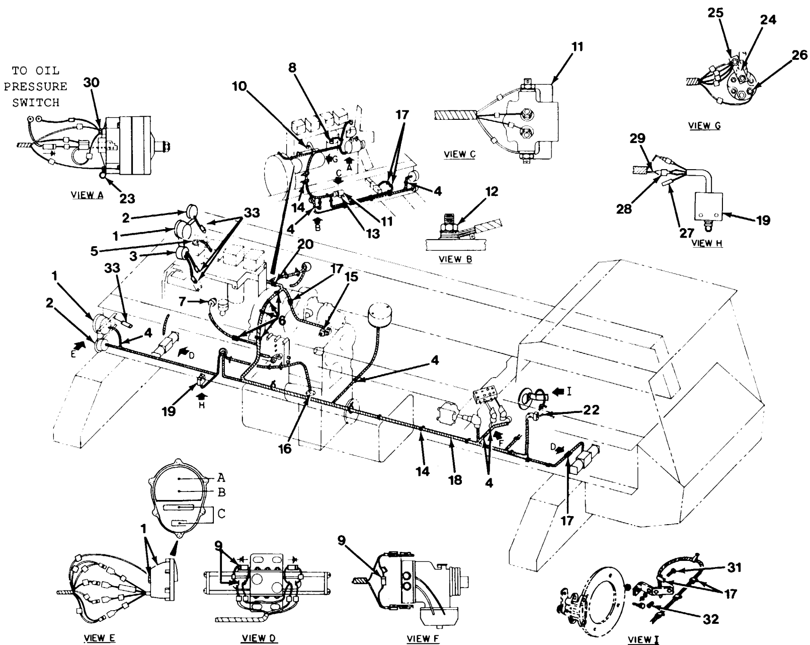
Figure 6-9. Rear Electrical.
