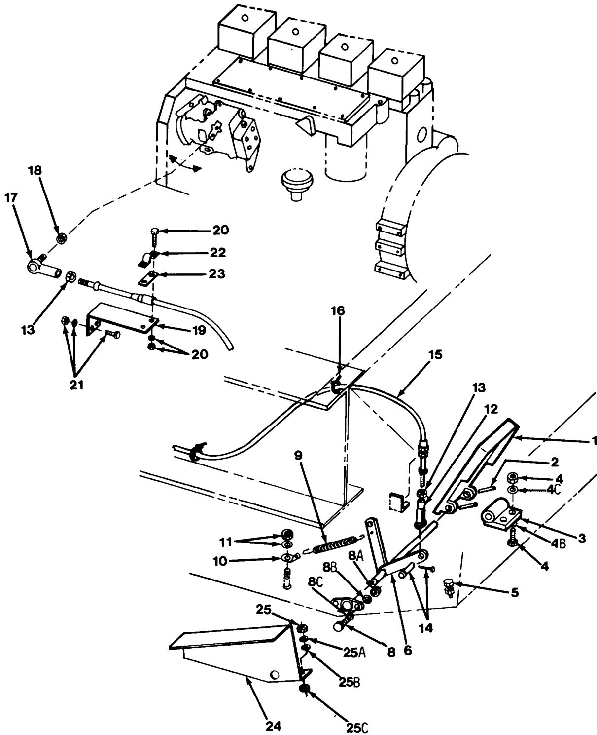
Figure 14-6. Throttle Control..
