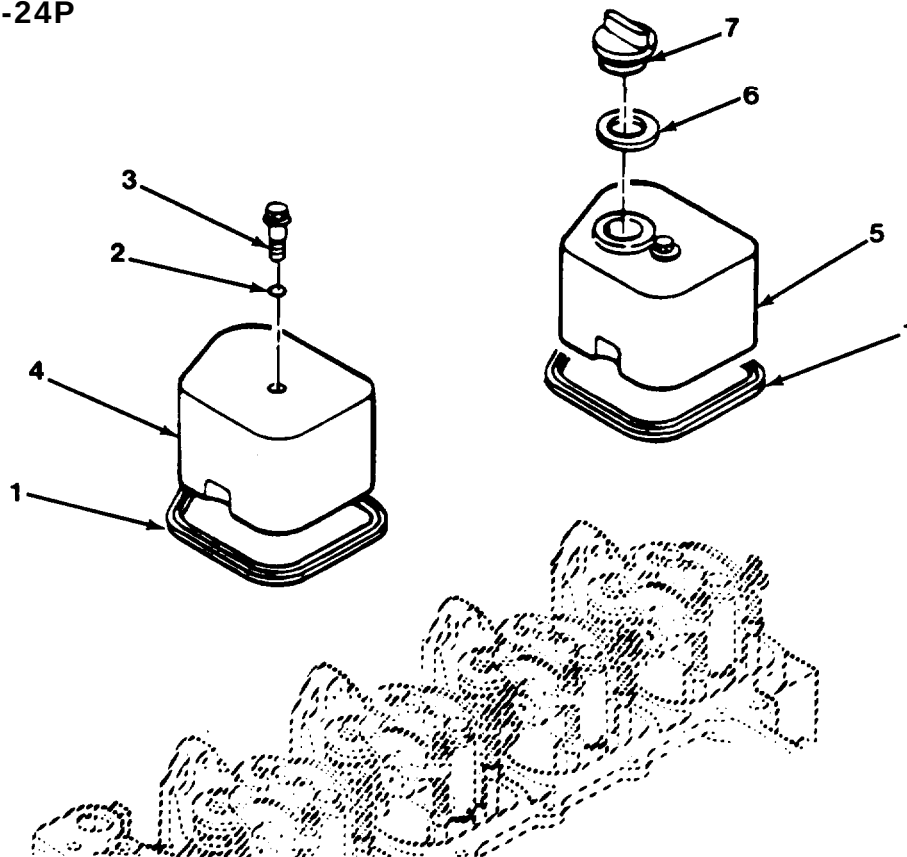
Figure 2-12. Valve cover.
