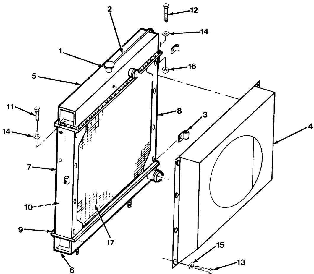
Figure 5-1A. Radiator.
