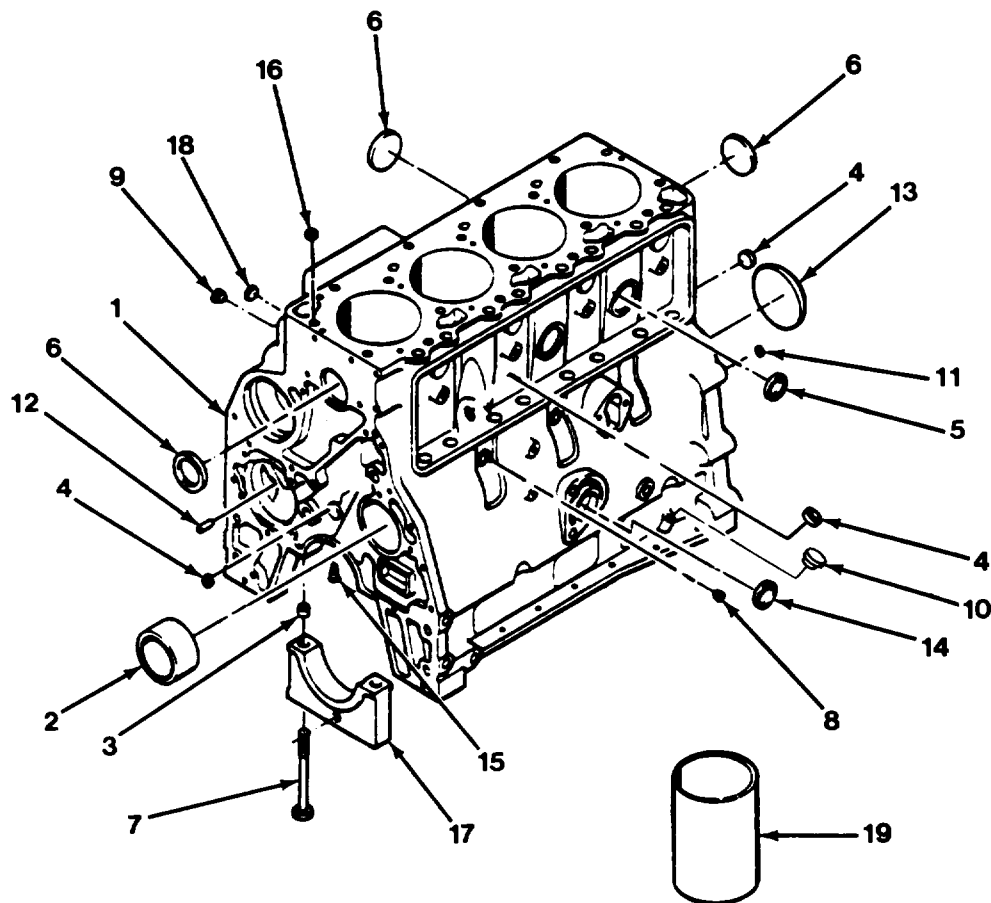
Figure 2-2. Cylinder Block .
