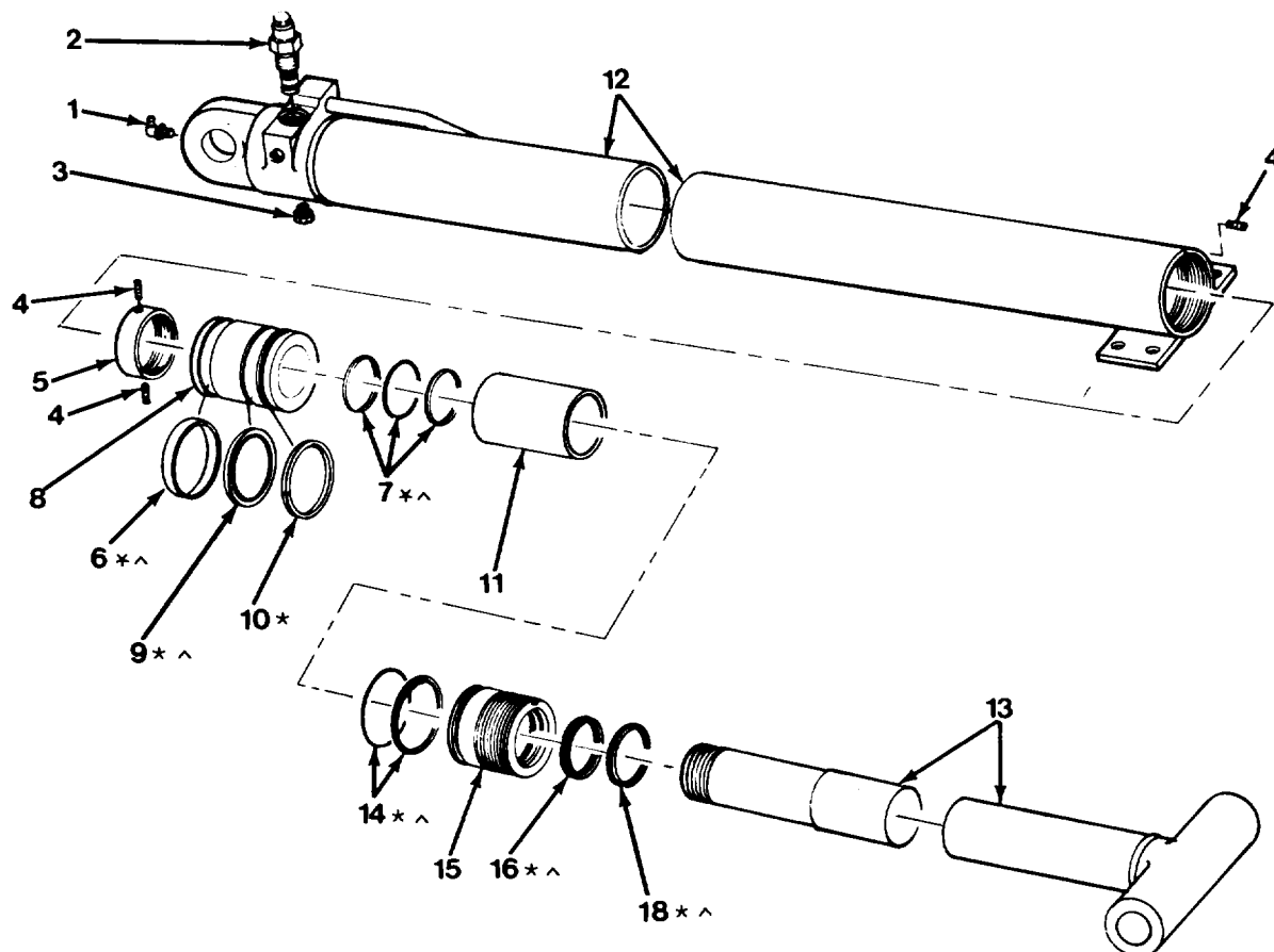
Figure 10-32 . Extend Cylinder.
