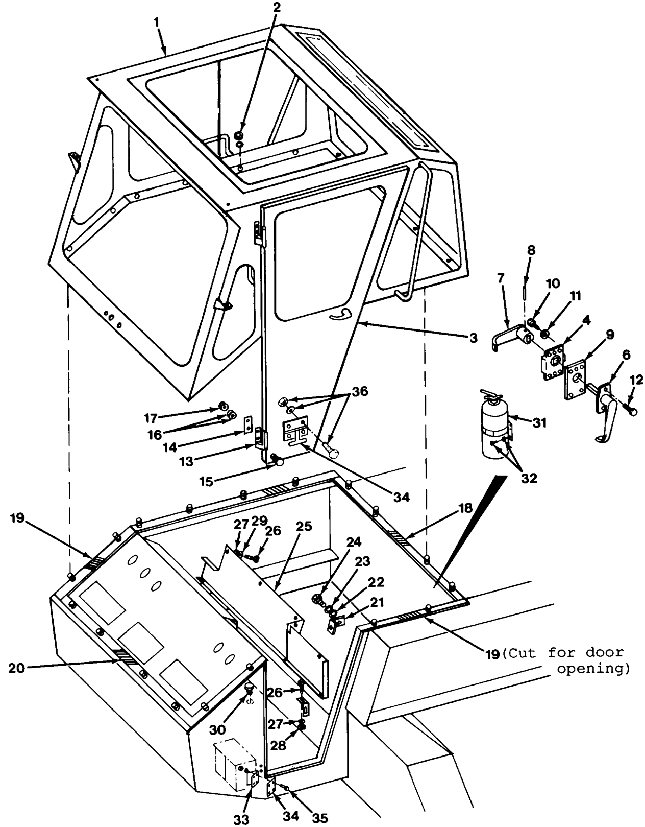
Figure 11-9. Operator's Cab.
