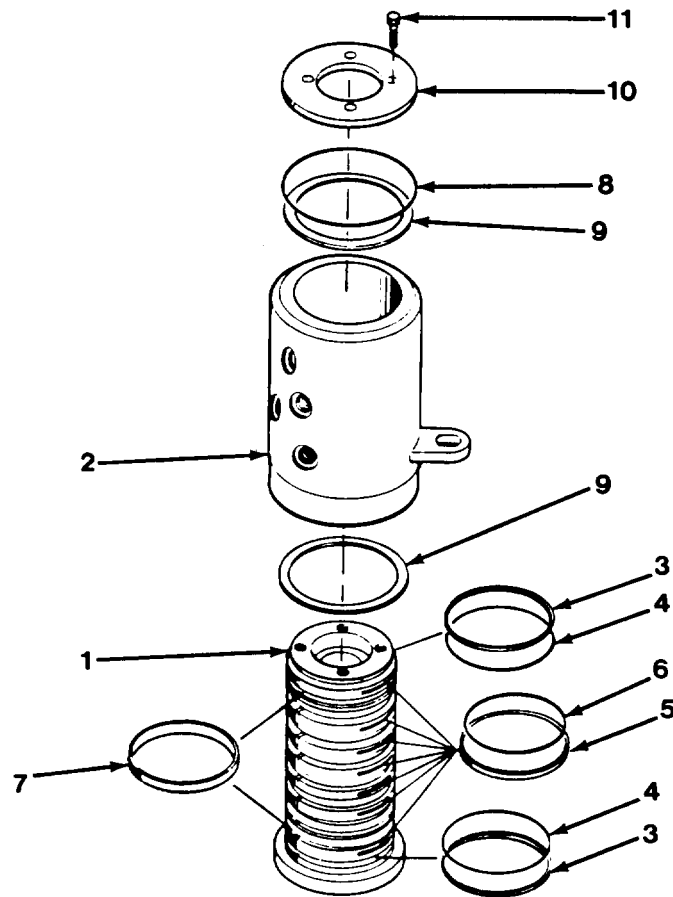
Figure 10-29. Rotary Manifold.
