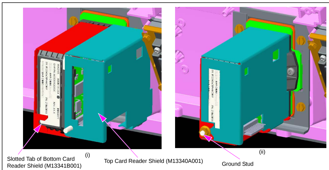
Figure 4: Positioning Top Card Reader Shield
