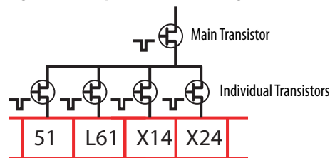
Figure 24 - Output Transistor Arrangement
