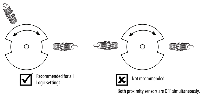
Figure 33 - Target Wheel Example 1
