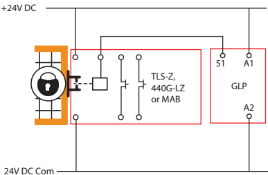
Figure 15 - Single TLS-Z, 440G-LZ, or MAB Connection
