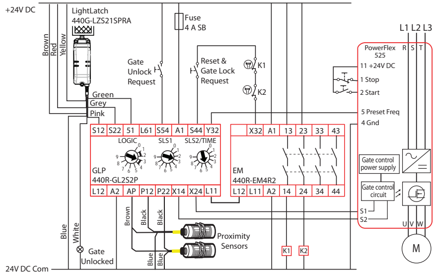
Figure 40 - Schematic for Safely Limited Speed Example
