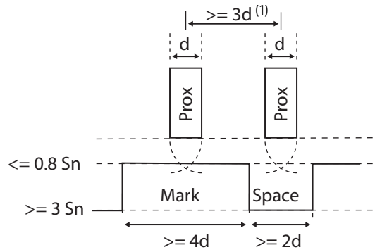
Figure 32 - Proximity Mark (Space Dimensions)
