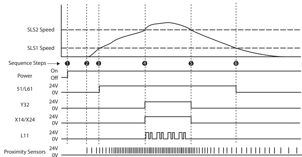
Figure 45 - Operational Sequence for Status Only Example
