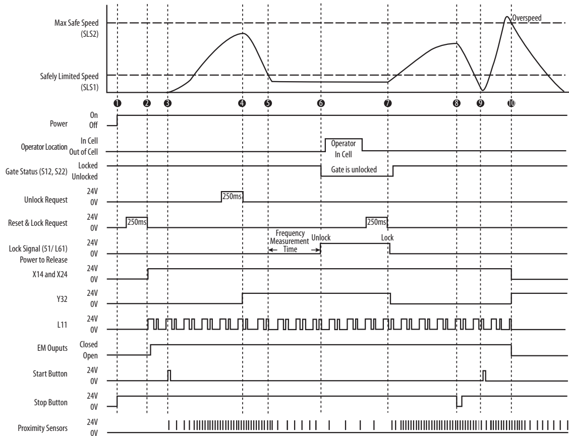
Figure 41 - Operational Sequence for Safely Limited Speed Example
