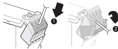
Figure 4 - Removable Terminals
