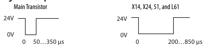
Figure 25 - Output Pulse Test Width
