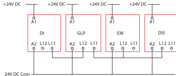
Figure 20 - Single Wire Safety Connections
