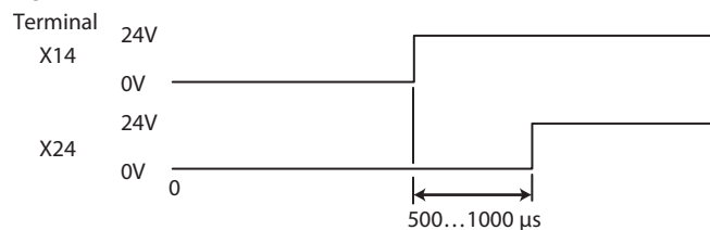
Figure 27 - OSSD Cross Fault Detection
