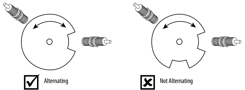
Figure 34 - Target Wheel Example 2
