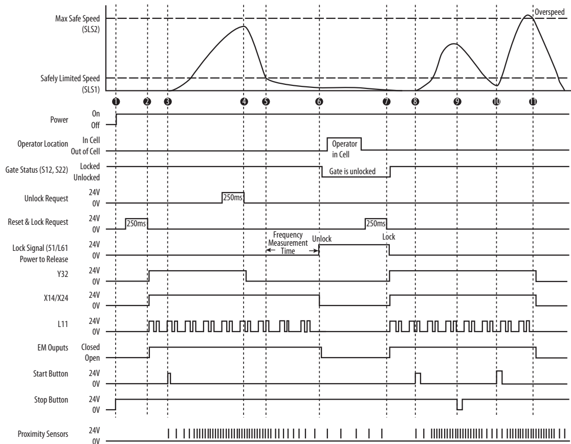
Figure 39 - Operational Sequence for Stop Cat 1 Example
