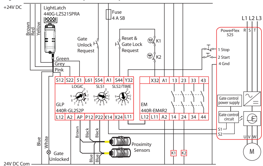
Figure 38 - Schematic for Stop Cat 1 Example
