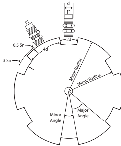
Figure 36 - Maximum Resolution
