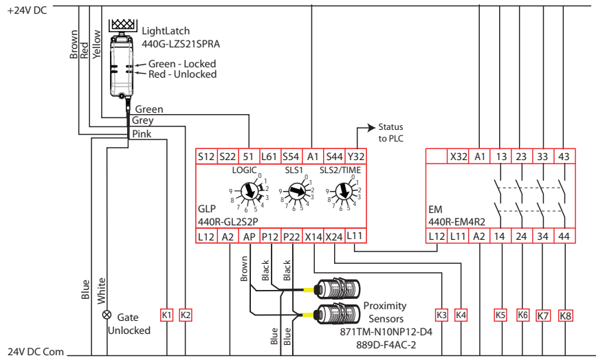
Figure 42 - Schematic for Delayed Unlock with Auto Reset
