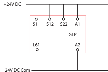
Figure 17 - No Guard Locking Connections
