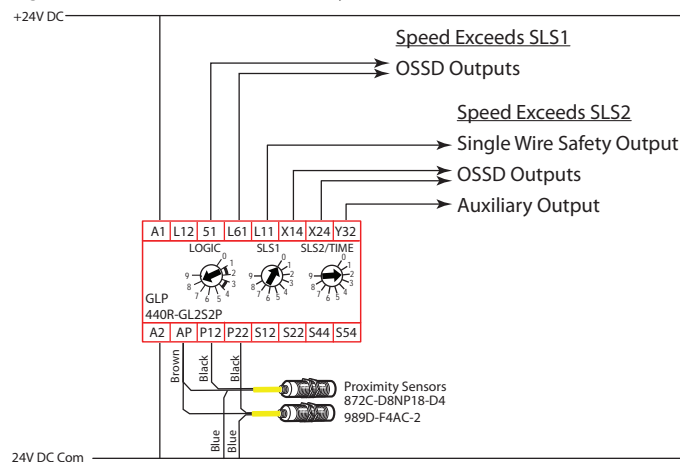
Figure 44 - Schematic for Status Only
