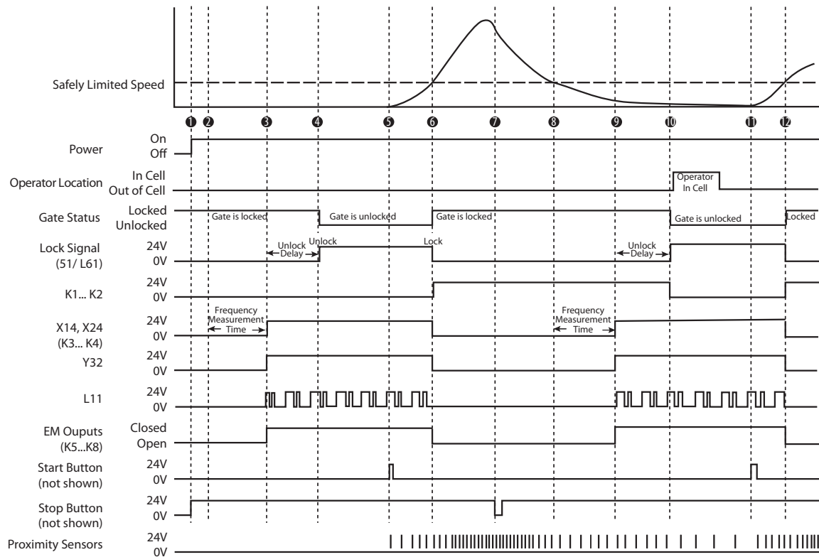
Figure 43 - Operational Sequence for Delayed Unlock with Auto Reset
