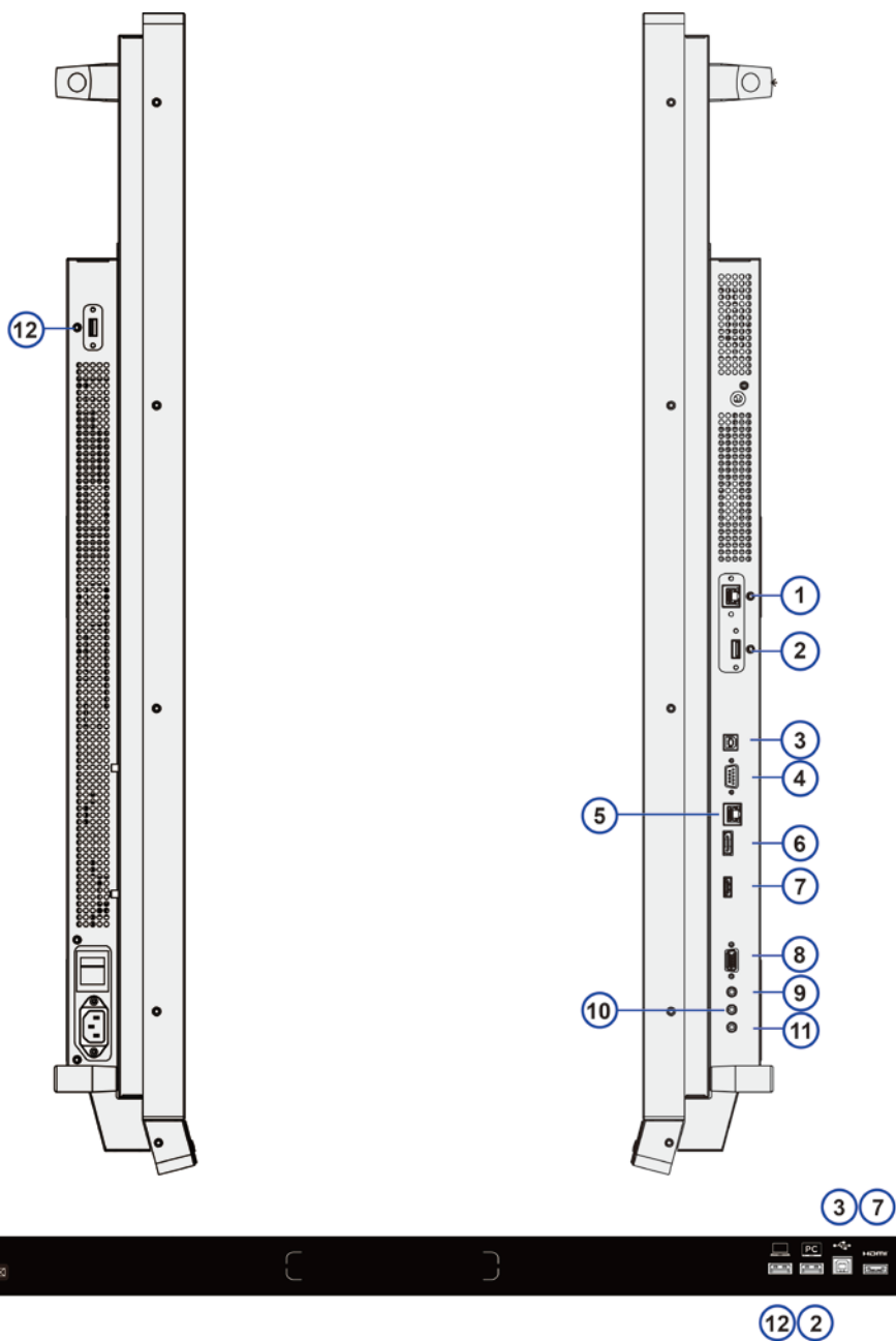
Figure 2-2. Display Input Panel Side/Front View
