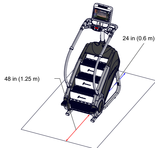
Fig. 1 Required Clearance
