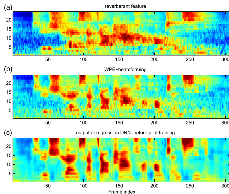
Fig. 8 An example of multi-channel front-end: a static LMFB features of one channel reverberant speech; b static LMFB features of WPE+Beamforming processed speech; c the output of front-end regression DNN: before joint training (estimated clean LMFB features)
