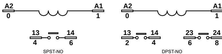
C3 - DIN/Panel Mount (Screw Terminals)
