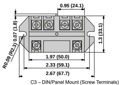
C3 - DIN/Panel Mount (Screw Terminals)
