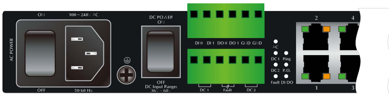
Figure 2-3: IGSW-24040T LED on Front Panel
