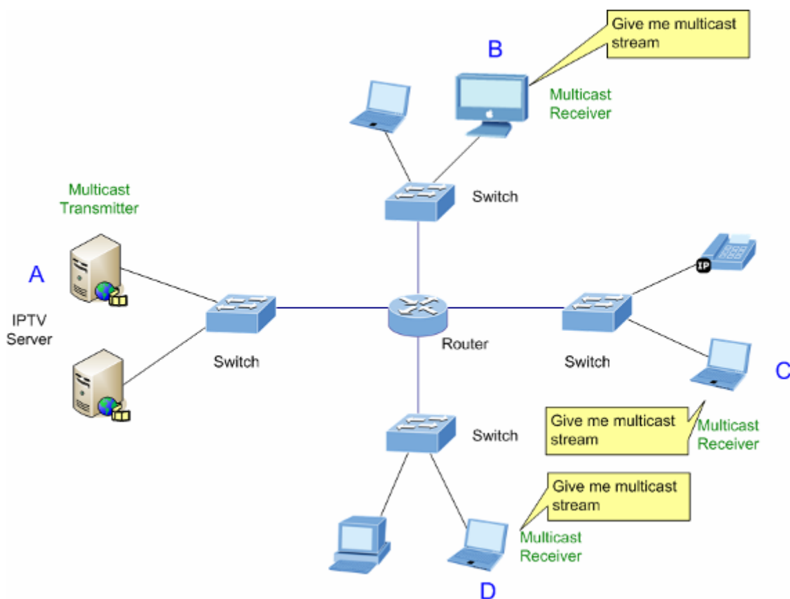
Figure 4-8-1: Multicast Service
