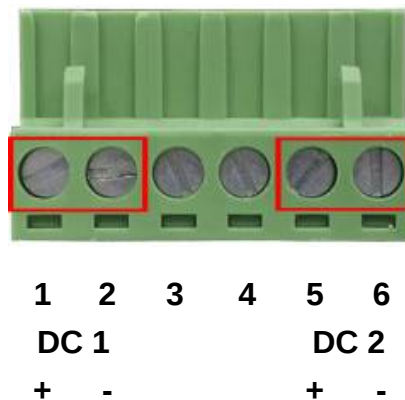
Figure 2-5 6-Pin Terminal Block Power Wiring Input
