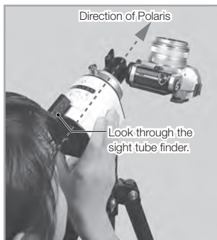
Direction of Polaris
