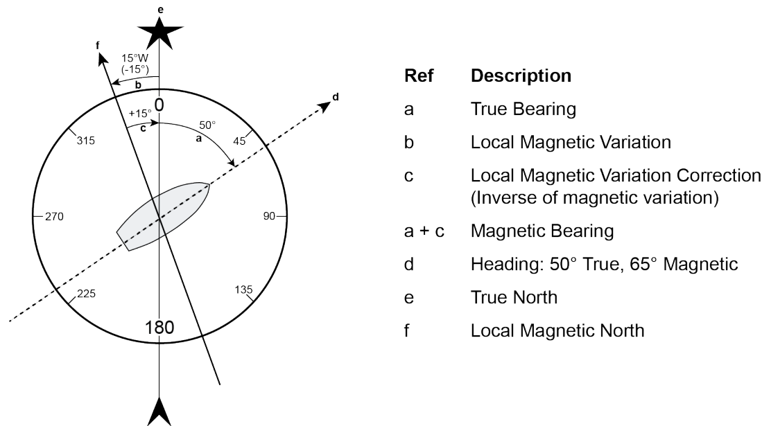
Figure 5: Illustration of Magnetic Variation and Correction
