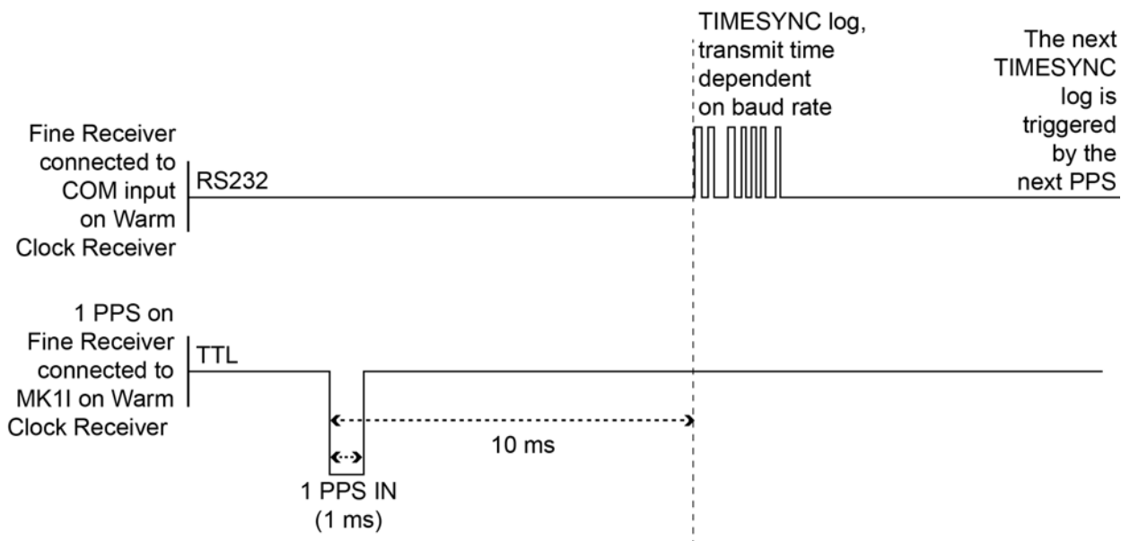
Figure 2: 1PPS Alignment
