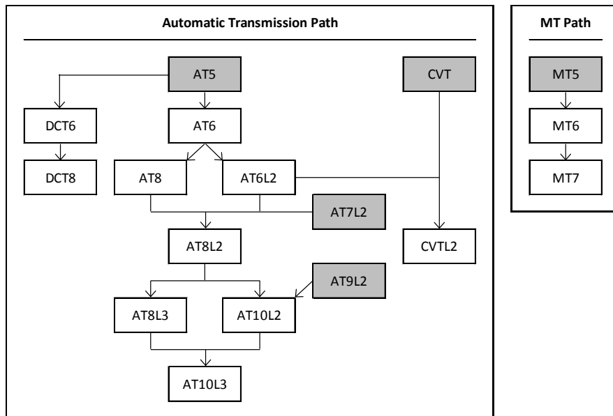
Figure 3. Transmission-Level Paths
