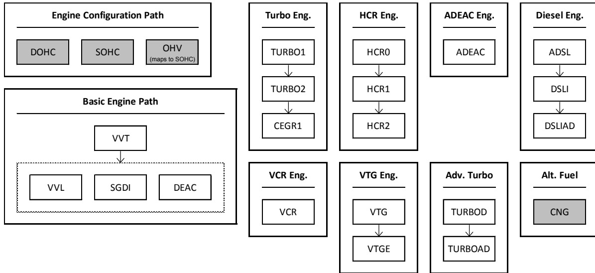
Figure 2. Engine-Level Paths
