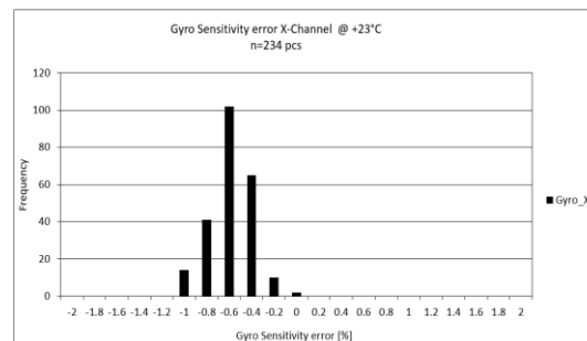
Chart 8 Gyro Sensitivity Error @ +23°C X-axis
