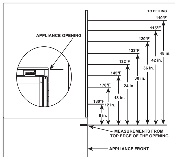
Figure 3.3. Maximum Wall Surface Temperatures Above Appliance
