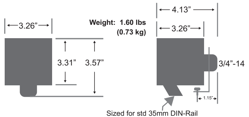
Figure 4: Dimensions and weight
