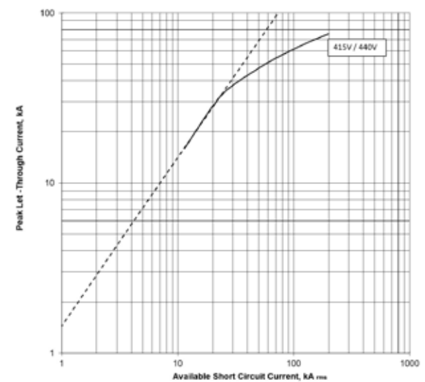
Let-through current I_D ; PDE3 ETU PXR10 LI; 630 A @ 415V and 440V
