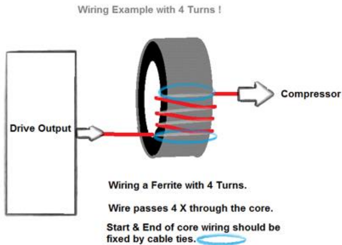
Figure 15: Example of good practice 4 turns with one ferrite
