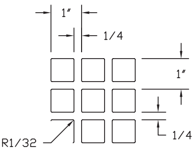
ENCLOSURE PERFORATION DETAIL
