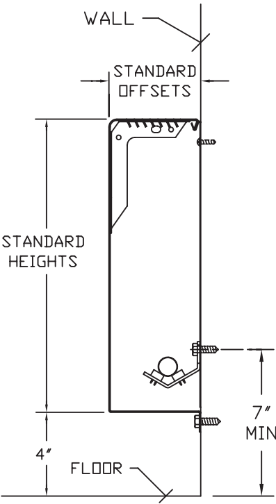
RETURN TO WALL, NO INLET LOUVERS DRAFT BARRIER STYLE RWDB
