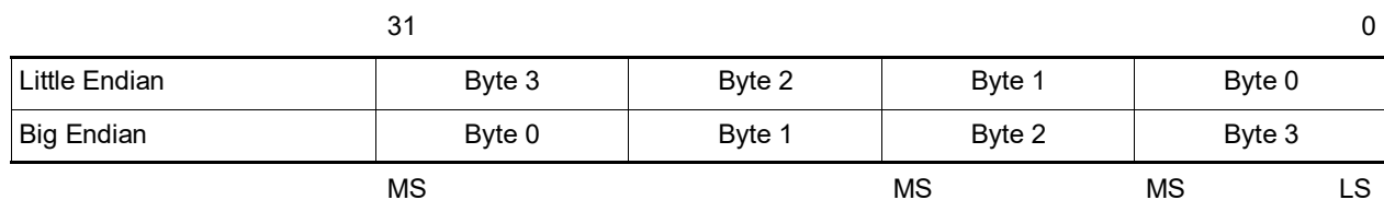
Figure 29. DXR Byte Locations
