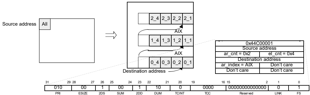
Figure E-3. Block-Synchronized 2-D (SUM=00b) to 2-D (DUM=10b)
