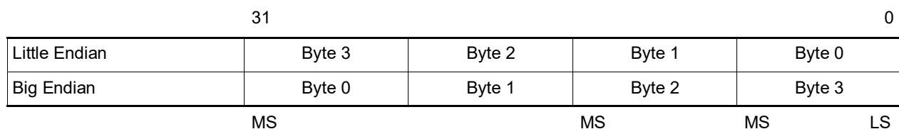
Figure 30. DRR Byte Locations
