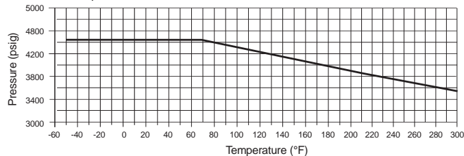
Pressure Limitations due to Fluid Temperature
