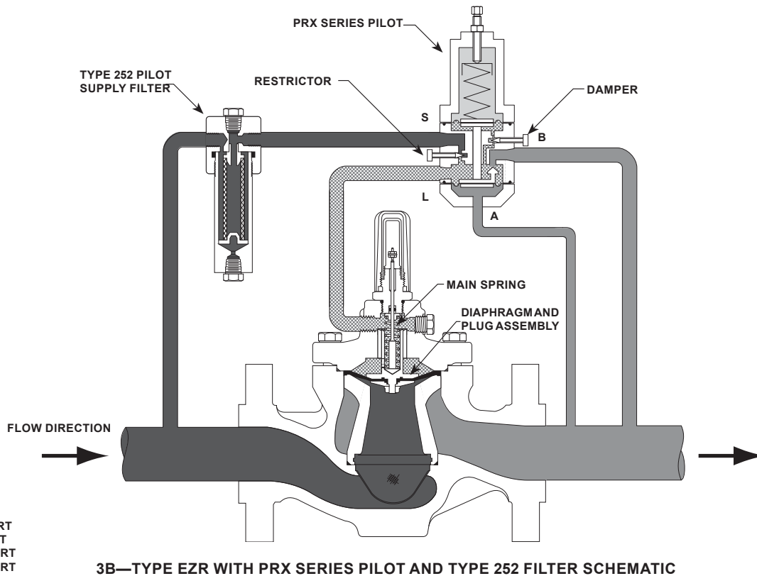
3B—TYPE EZR WITH PRX SERIES PILOT AND TYPE 252 FILTER SCHEMATIC
